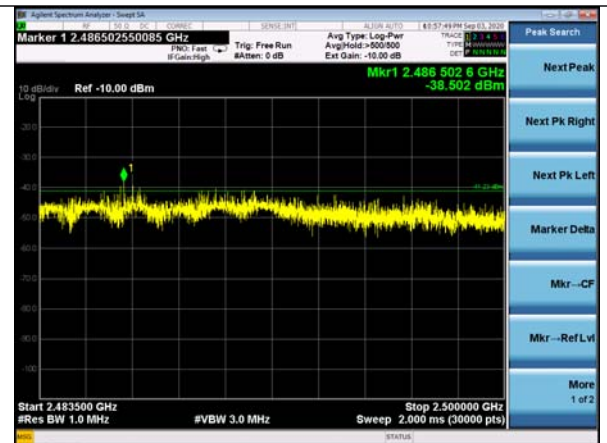
UBE, Hopping
