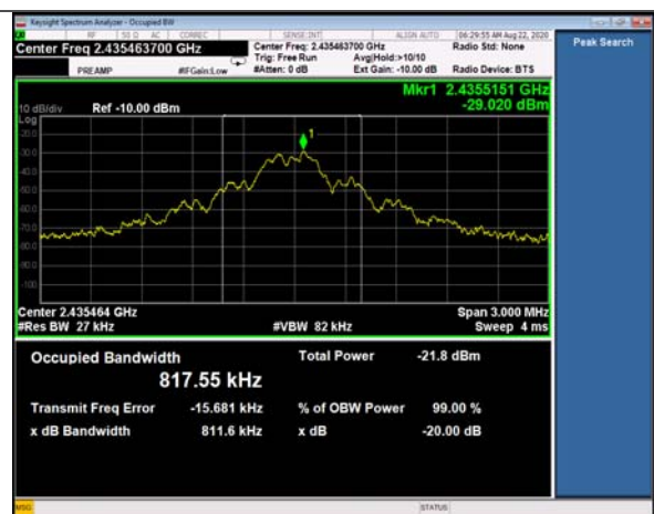
Mid Channel
