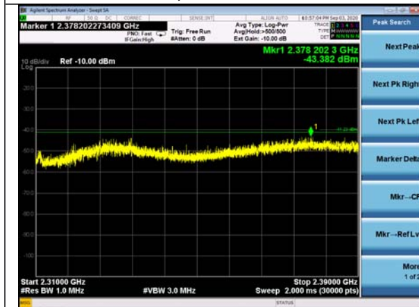
LBE, Hopping
