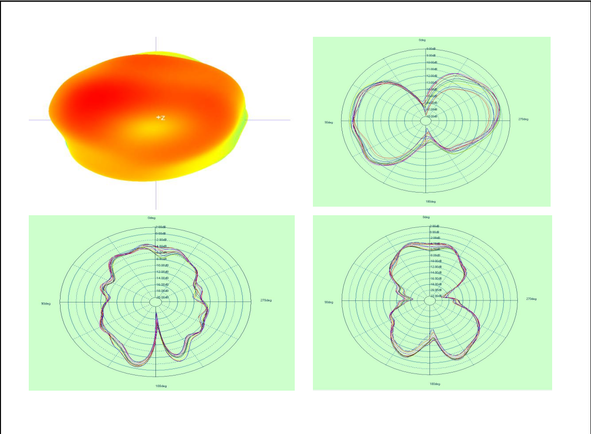
Antenna Radiation Pattern
