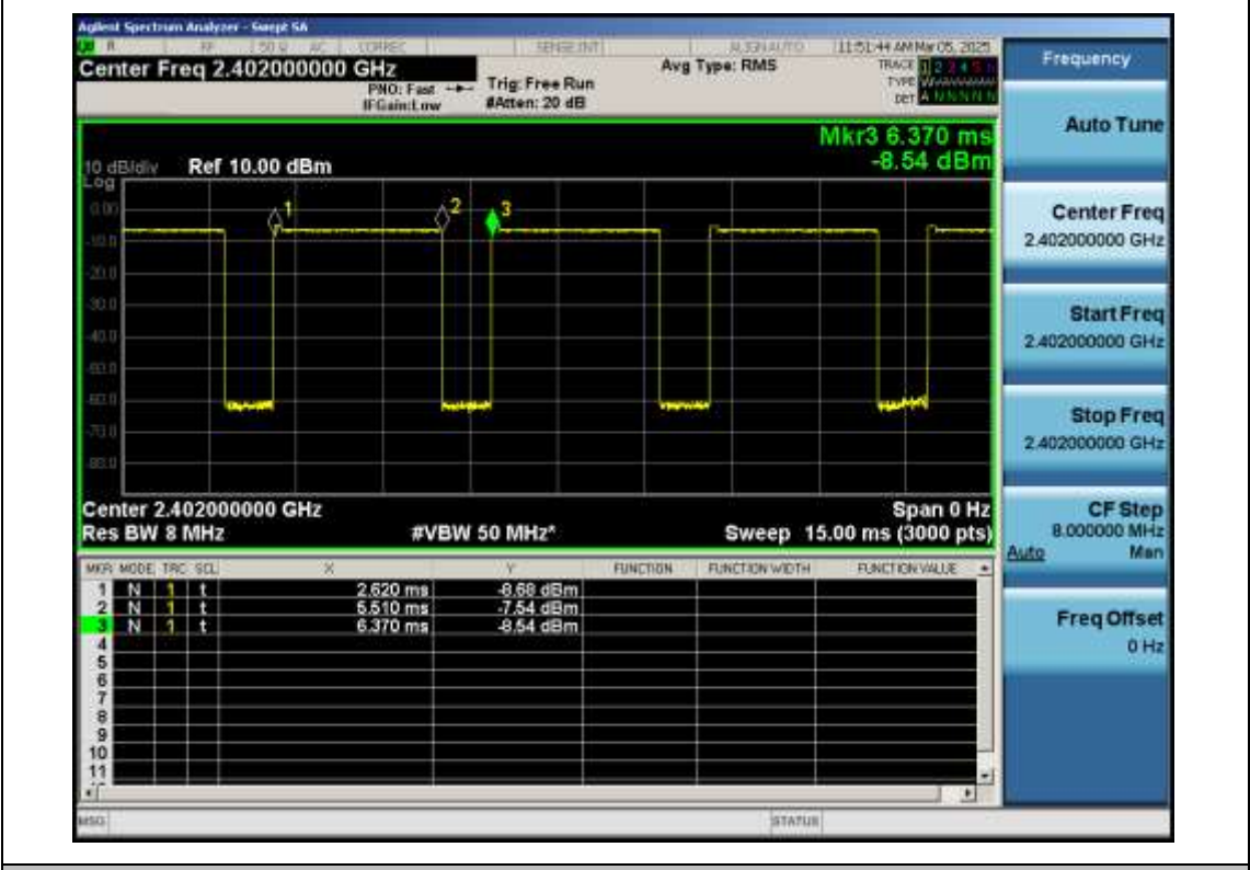
EDR-π /4-DQPSK-Ant1-2402
