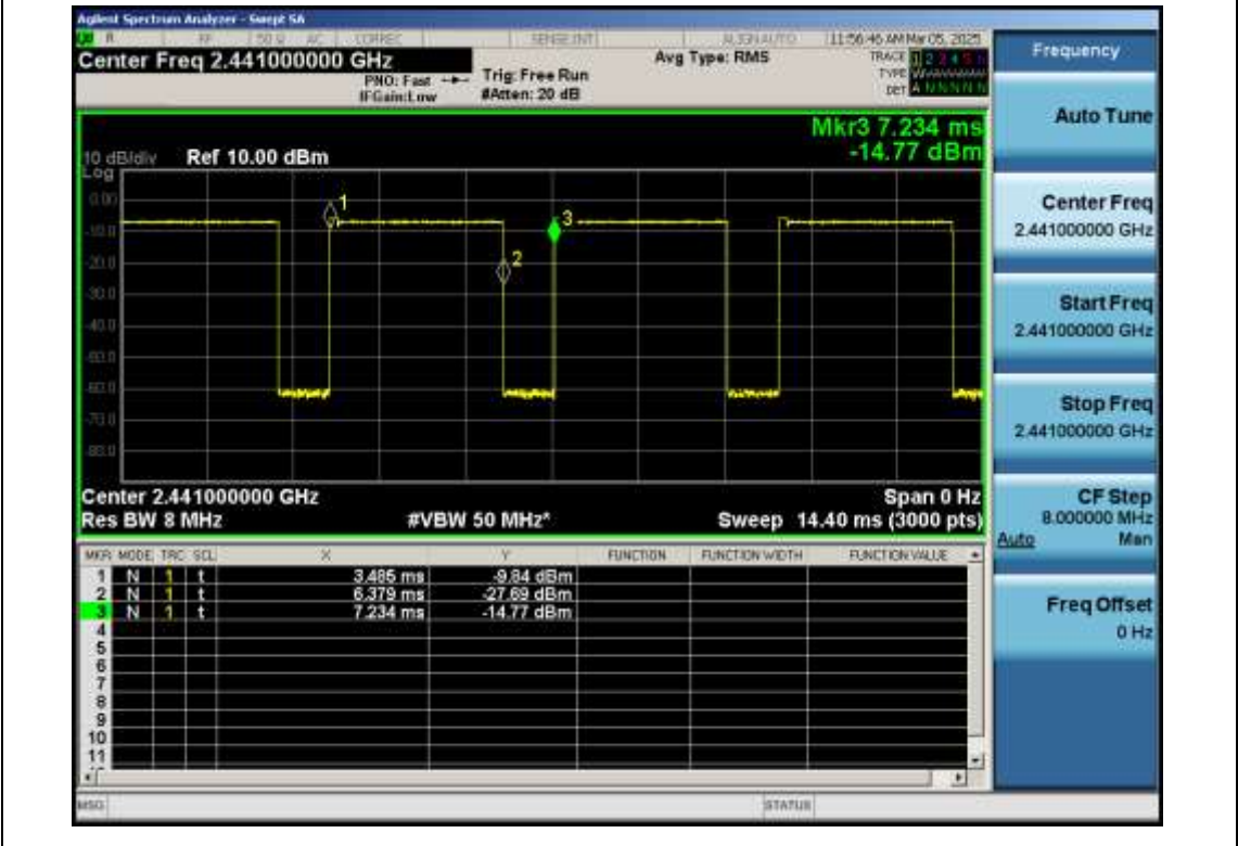
EDR-8DPSK-Ant1-2441
