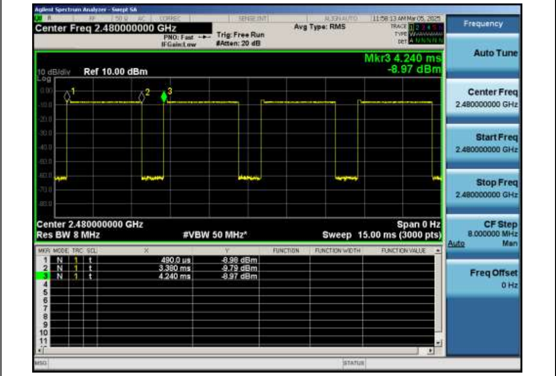
EDR-π /4-DQPSK-Ant1-2480
