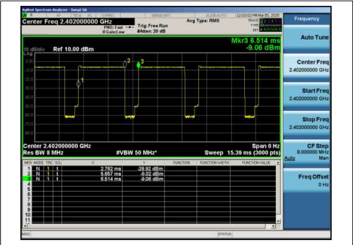
EDR--8DPSK-Ant1-2402
