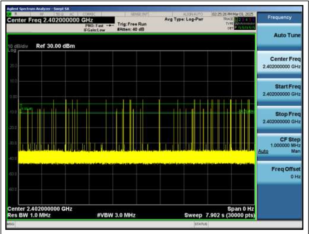
Test_Graph_EDR_HOP_ANT1_NA_2Mbps_2402_Number of Burst
