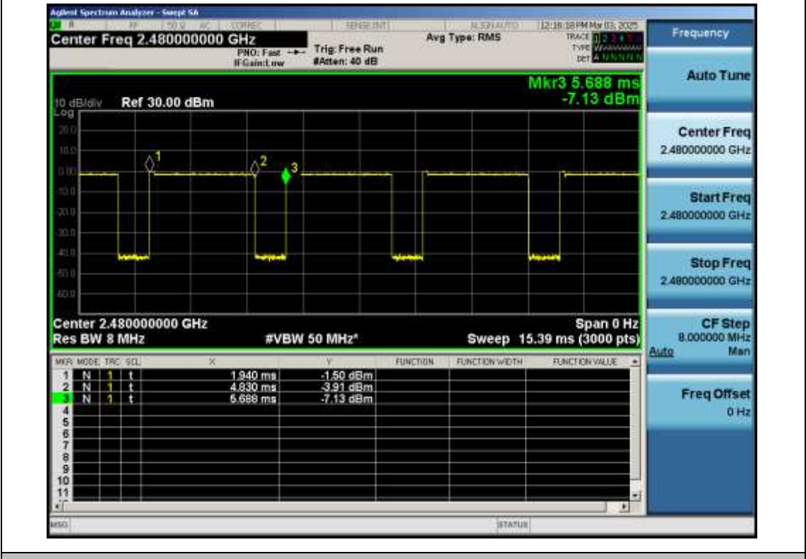
EDR-π /4-DQPSK-Ant1-2480
