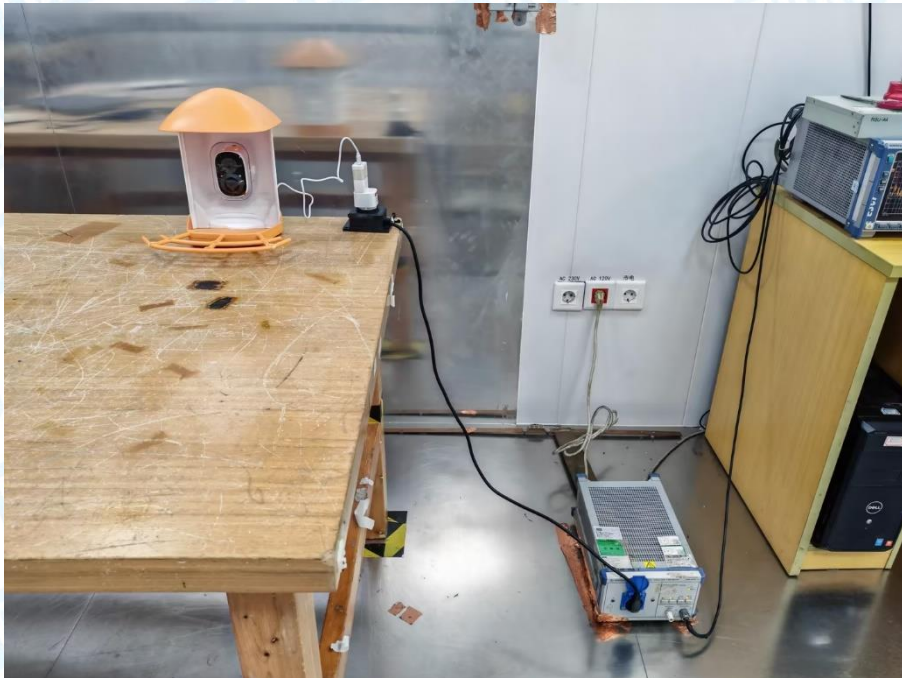
Photo of Setup for Radiated Emission (30MHz~1GHz)
