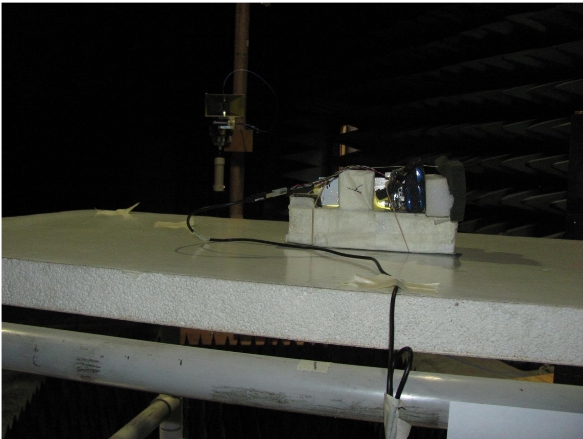
The EUT was mounted on a foam stand in order to change its orientation.
