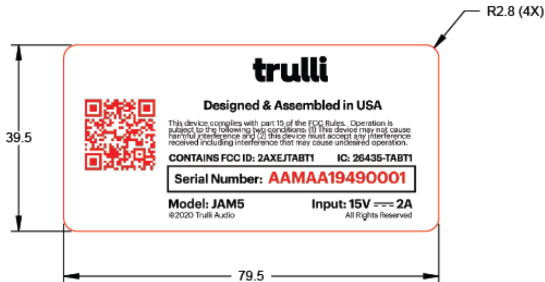
Drawing of Label
