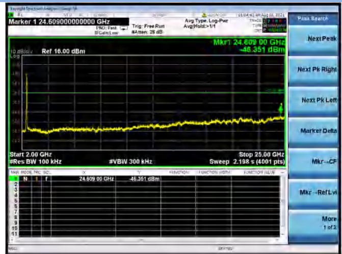
802.11n-40 MIDDLE CHANNEL, SPURIOUS 2 GHz ~ 25 GHz
