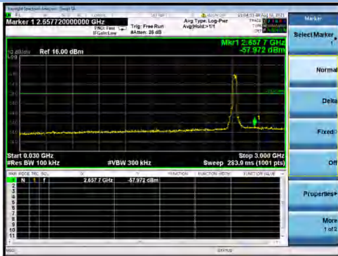
802.11n-40 HIGH CHANNEL CARRIER LEVEL
