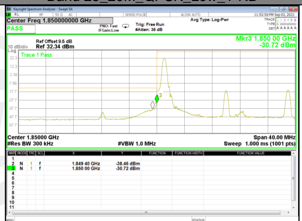
Band 25_20M_QPSK_Low_Full-RB
