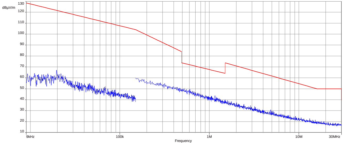
Plot 1: 9 kHz to 30 MHz, 2402 MHz, transmit mode, valid for 1 Msps and 2 Msps
