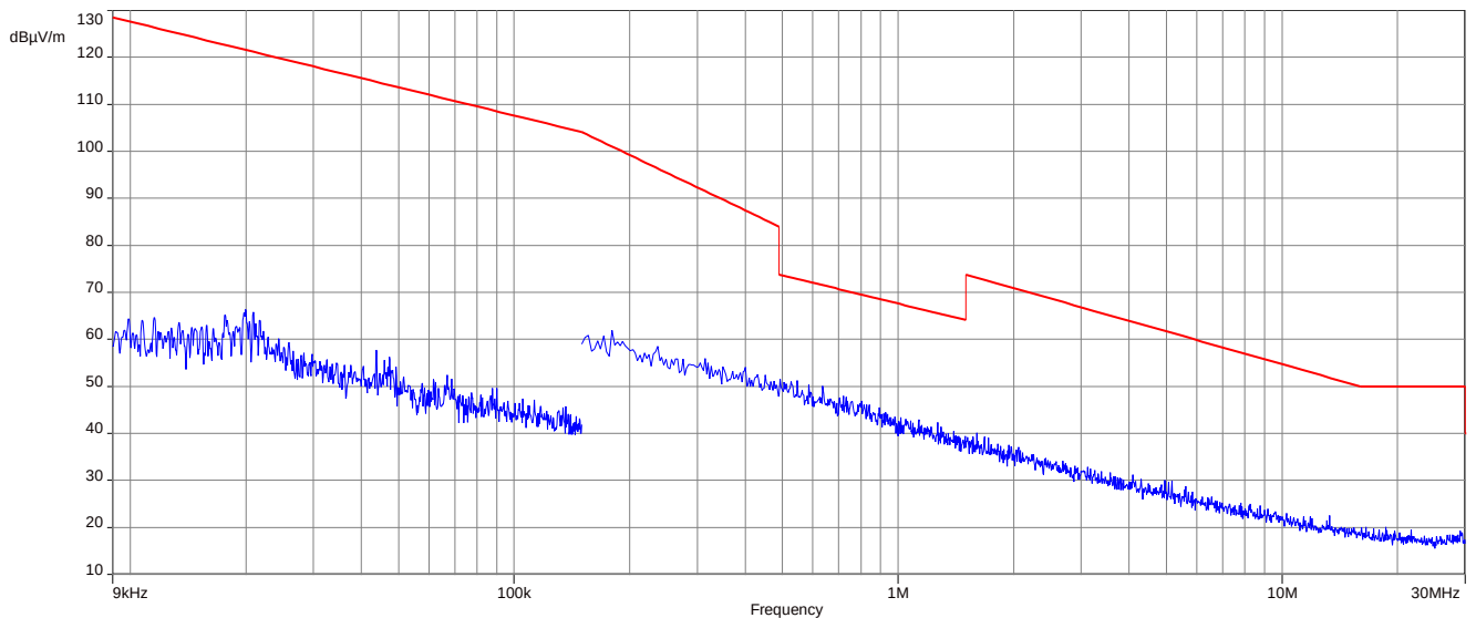
Plot 2: 9 kHz to 30 MHz, 2440 MHz, transmit mode, valid for 1 Msps and 2 Msps
