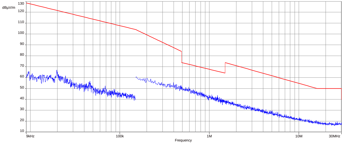
Plot 3: 9 kHz to 30 MHz, 2480 MHz, transmit mode, valid for 1 Msps and 2 Msps
