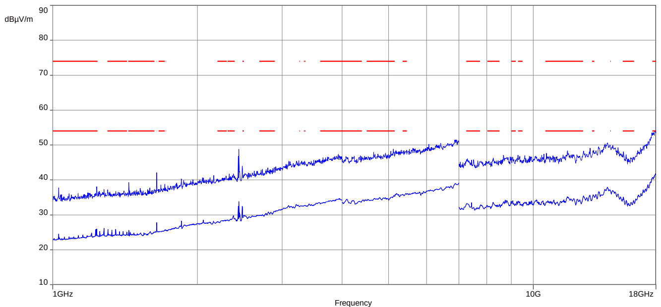
Plot 6: 1 GHz to 18 GHz, TX mode, 2480 MHz, vertical & horizontal polarization, 2 Msps
