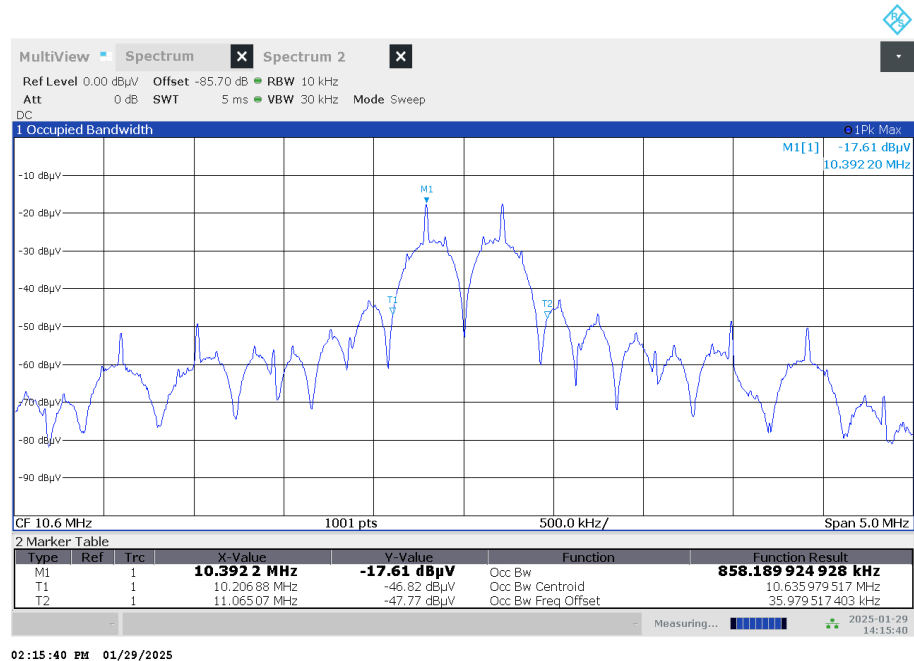
Plot 1: 212 kBit/s, 99 % emission bandwidth
