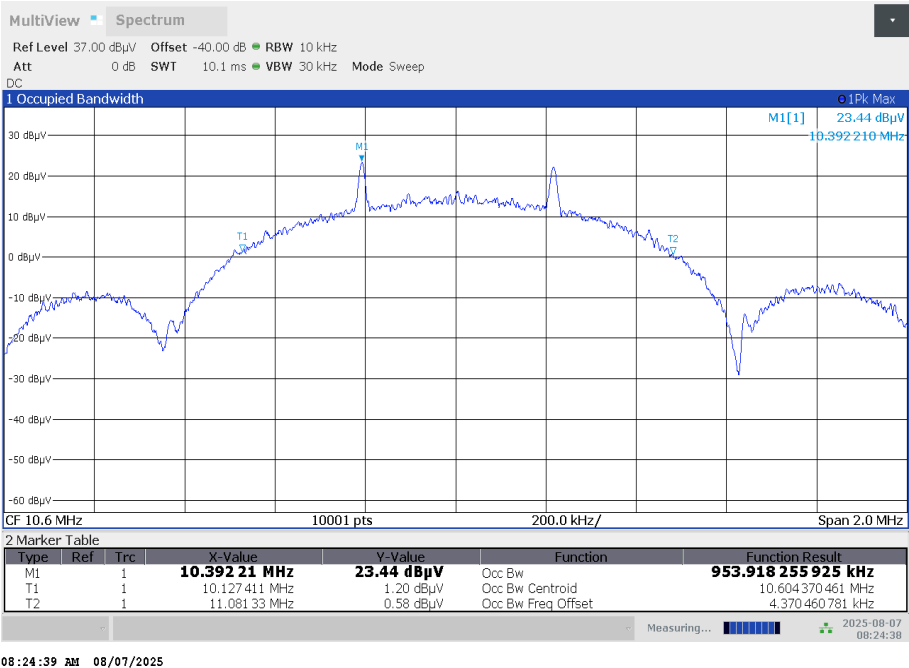
Plot 2: 424 kBit/s, 99 % emission bandwidth
