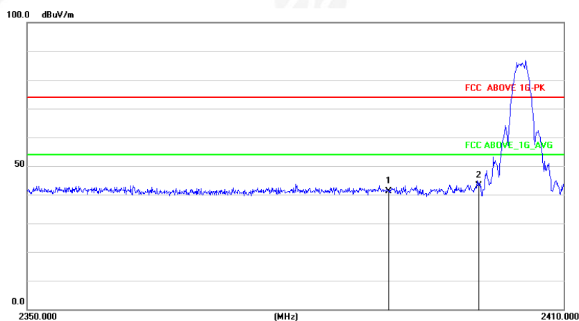
2402MHz Horizontal
