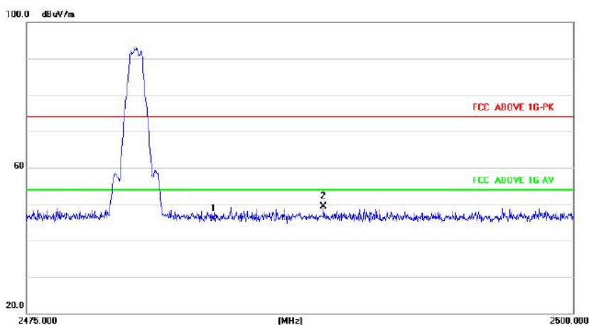
2480MHz Vertical
