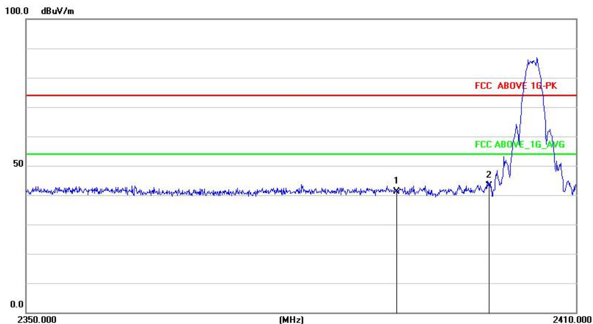
2402MHz Horizontal
