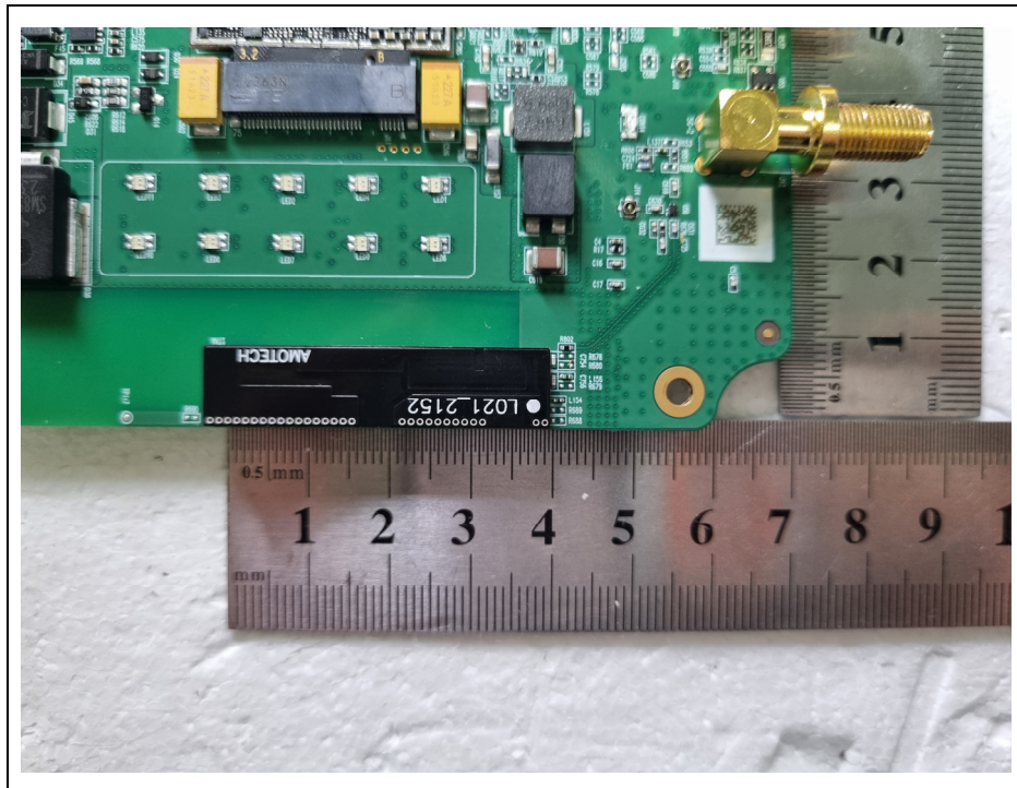
< 5GNR, LTE Antenna 1 >
