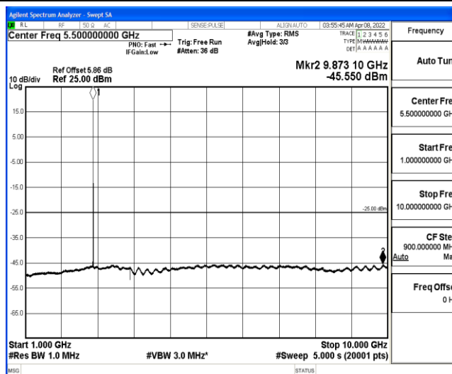
Band41-5MHz-16QAM-41565-1RB#0-Range4:1000~10000MHz
