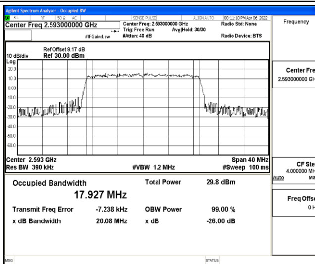
Band41-20MHz-16QAM-41490-100RB#0
