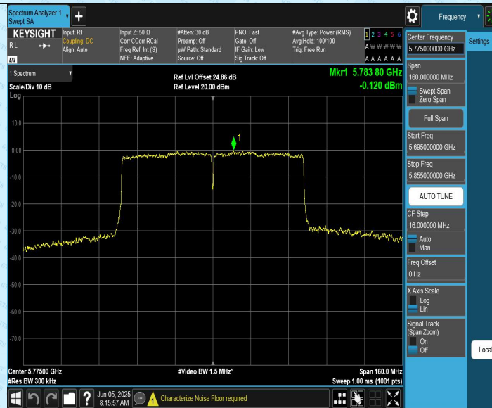
11AC80CDD_Ant2_5775
