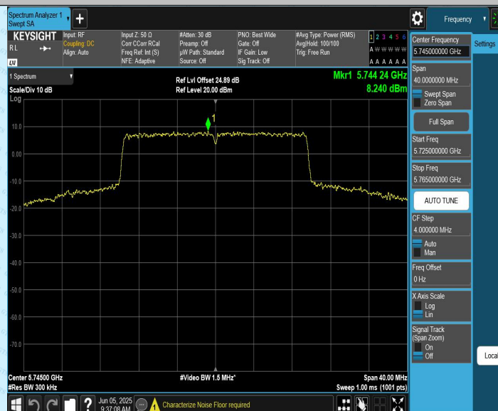
11AX20CDD_Ant2_5745
