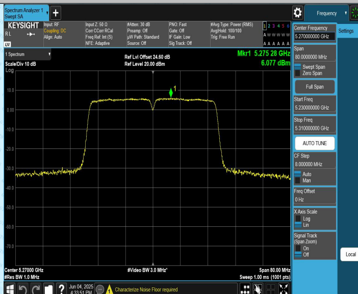
11AC40CDD_Ant2_5270
