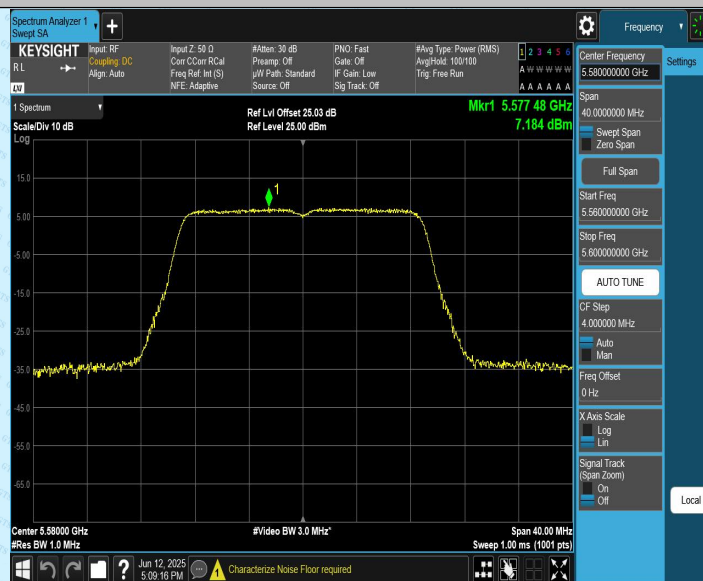
11AC20CDD_Ant2_5580
