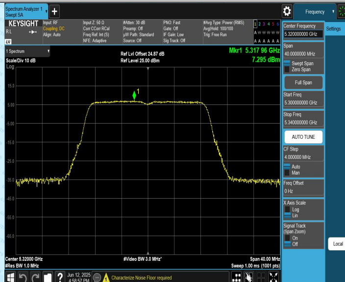
11AC20CDD_Ant2_5320
