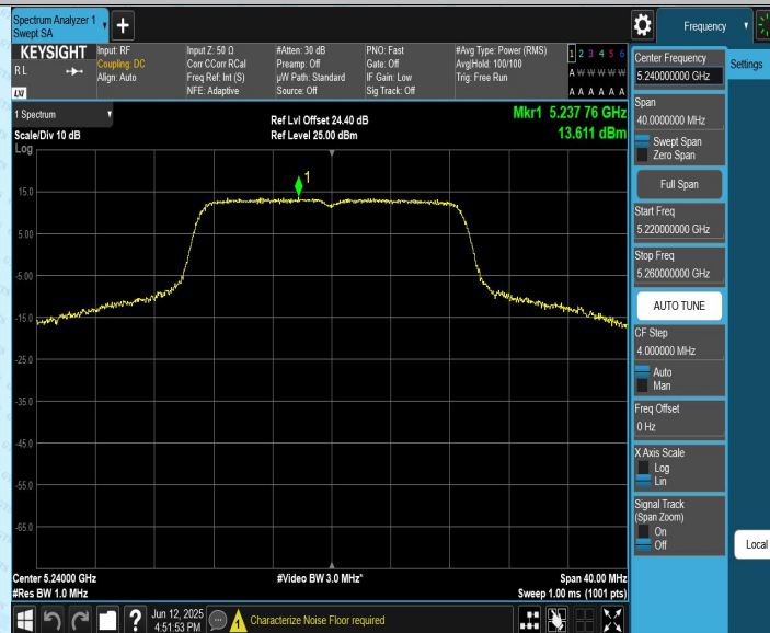
11AC20CDD_Ant2_5240
