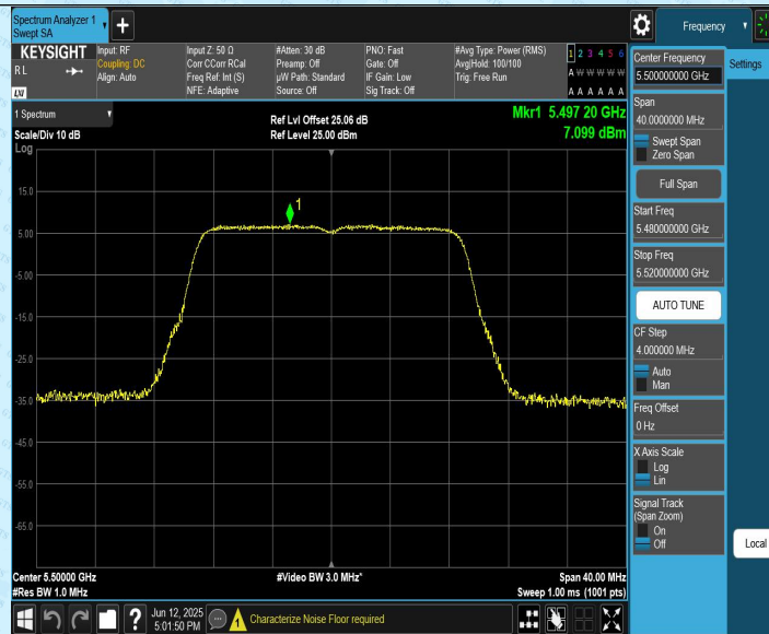
11AC20CDD_Ant2_5500
