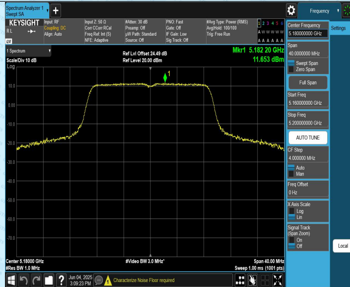
11AC20CDD_Ant2_5180
