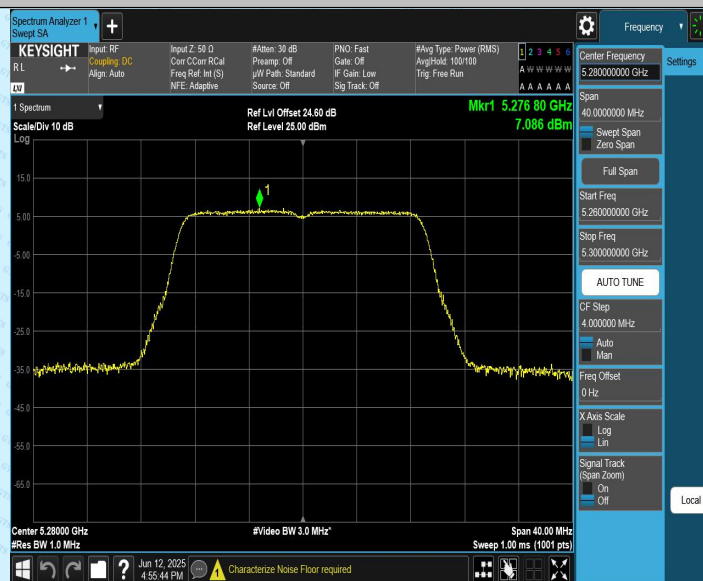
11AC20CDD_Ant2_5280
