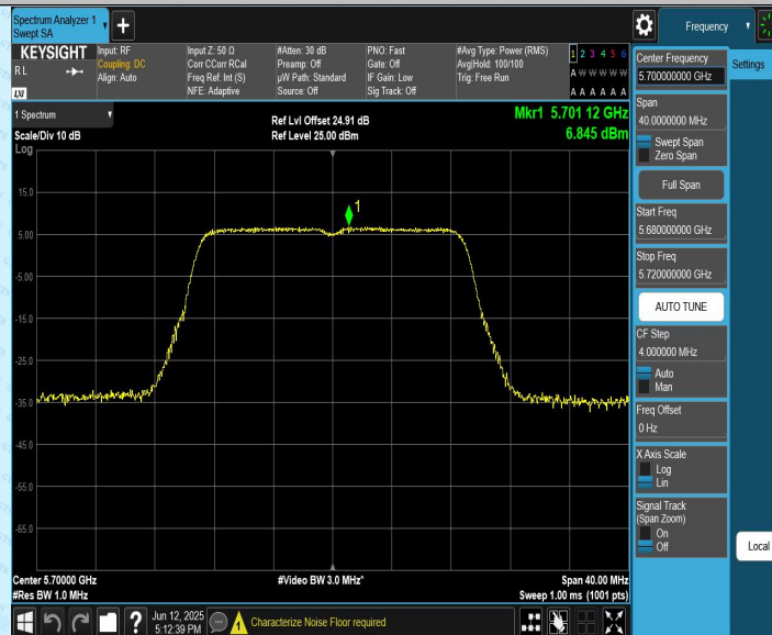
11AC20CDD_Ant2_5700
