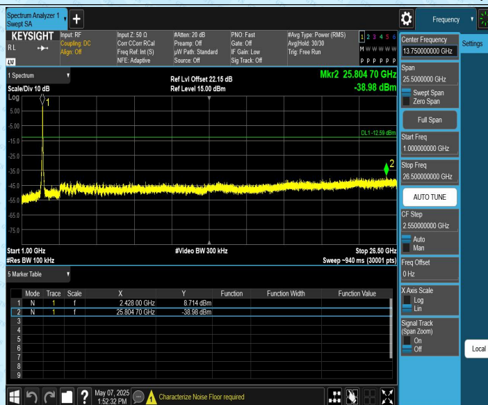
11AX40CDD_Ant1_2437_0~Reference
