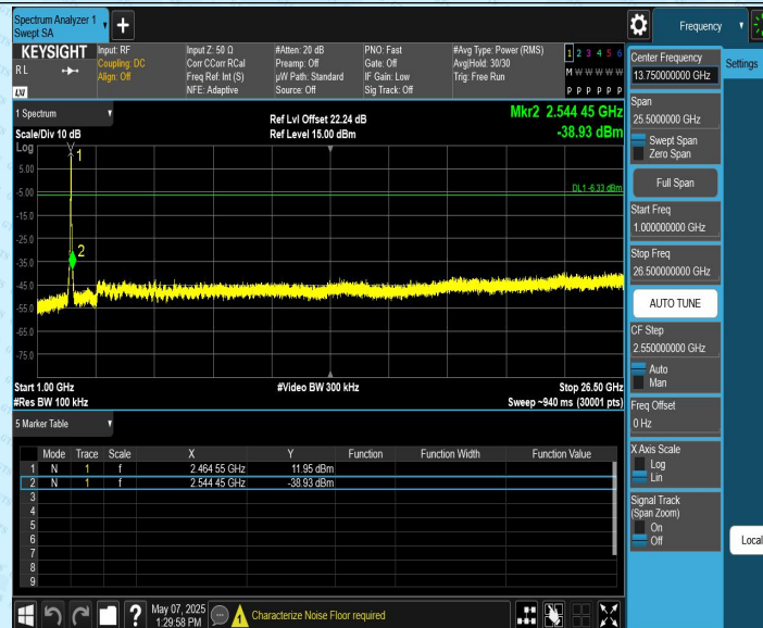
11AX20CDD_Ant2_2462_0~Reference
