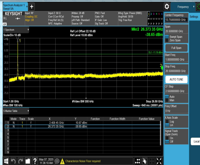
11AX20CDD_Ant2_2412_0~Reference
