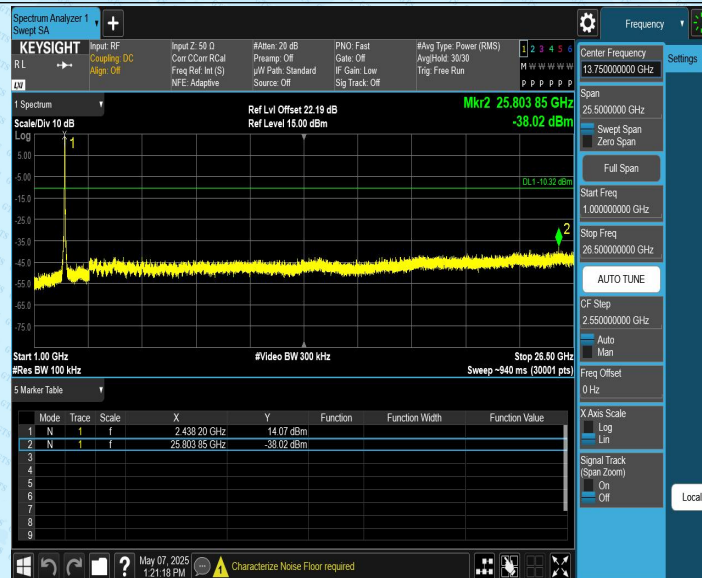
11AX20CDD_Ant2_2437_0~Reference
