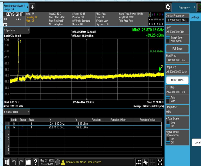
11G-CDD_Ant2_2412_0~Reference
