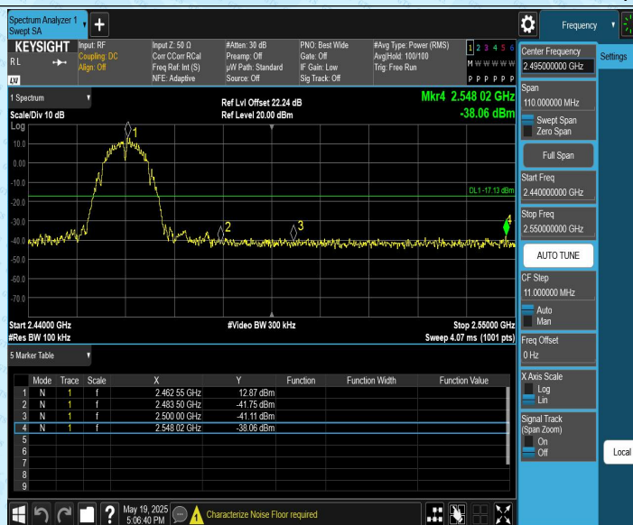
11B-CDD_Ant2_High_2462
