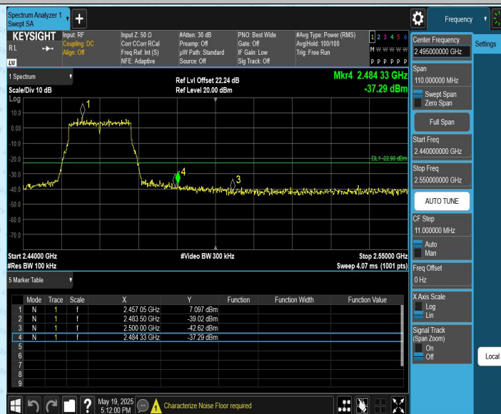
11N20CDD_Ant2_High_2462
