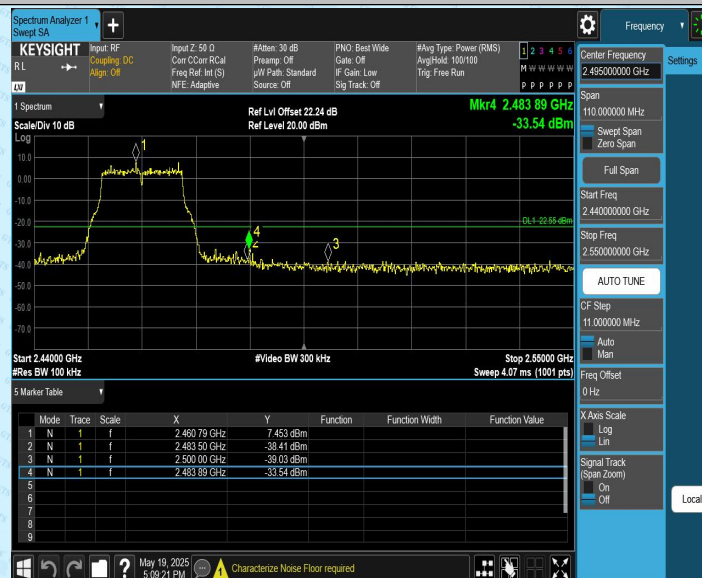
11G-CDD_Ant2_High_2462
