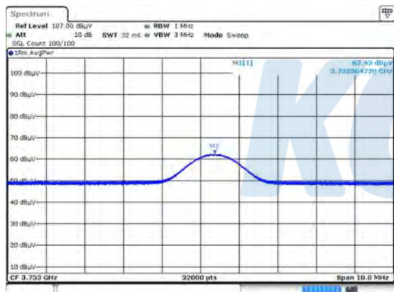
Average data (3 733.36 MHz)
