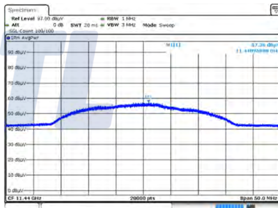
Average data (11 440.96 MHz)
