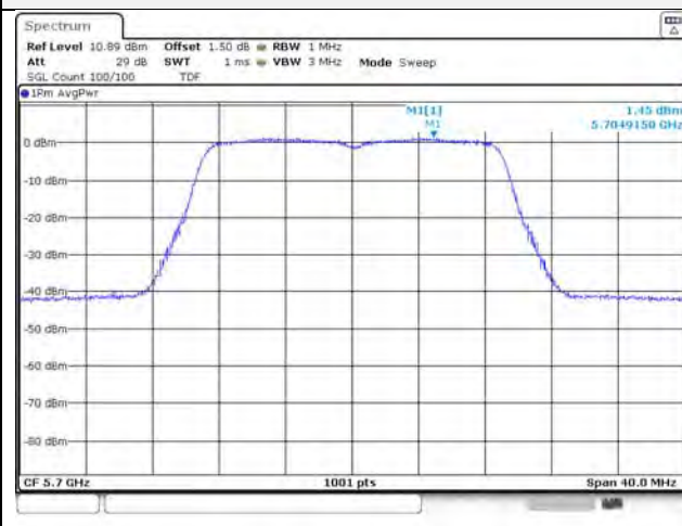
UNII-2C / 802.11n HT20 / 5 700 MHz
