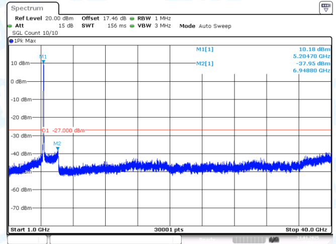
11AC80-CDD-Ant2-5210-1000~40000-PASS
