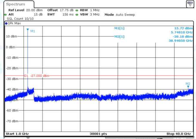
11AC20-CDD-Ant2-5745-1000~40000-PASS
