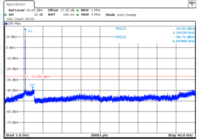
11AC20-CDD-Ant2-5180-1000~40000-PASS
