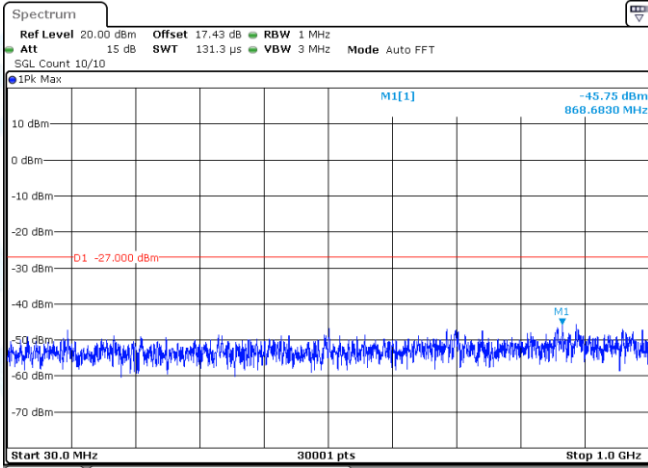
11AC20-CDD-Ant1-5320-30~1000-PASS
