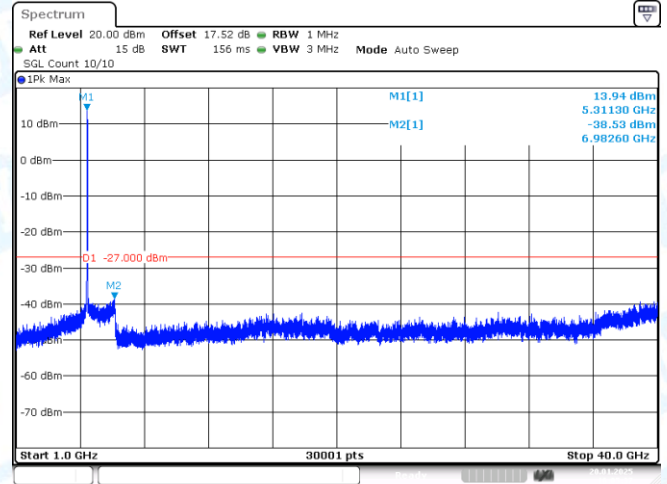
11AC40-CDD-Ant2-5310-1000~40000-PASS
