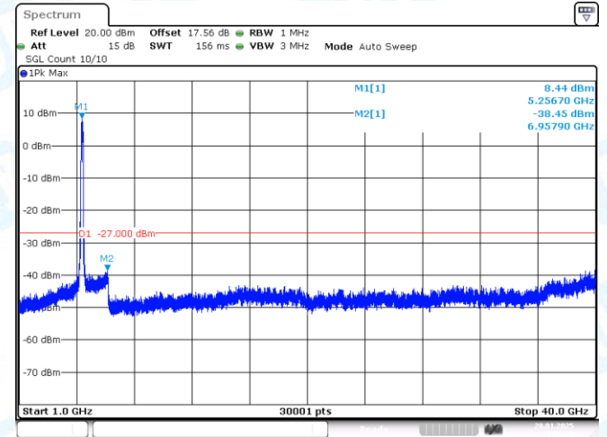
11AC160-CDD-Ant2-5250-1000~40000-PASS
