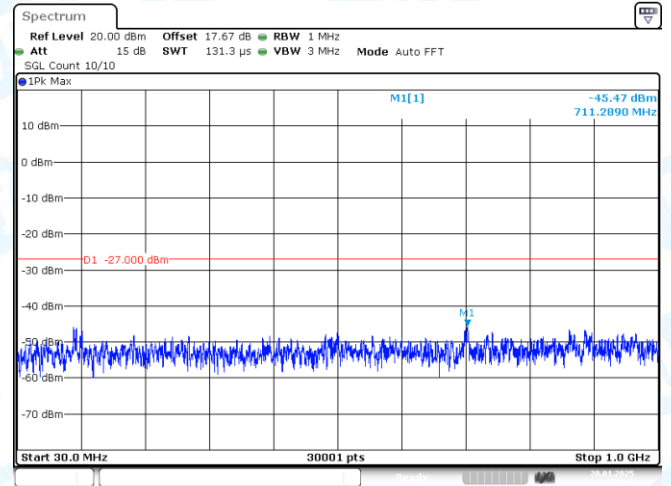
11AC40-CDD-Ant2-5550-30~1000-PASS
