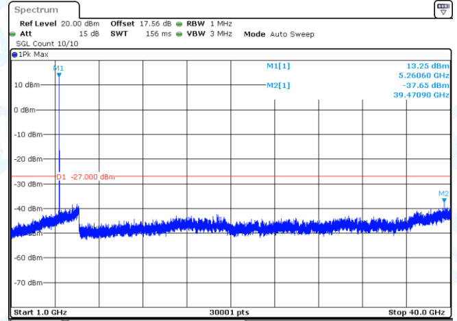
11AC20-CDD-Ant2-5260-1000~40000-PASS
