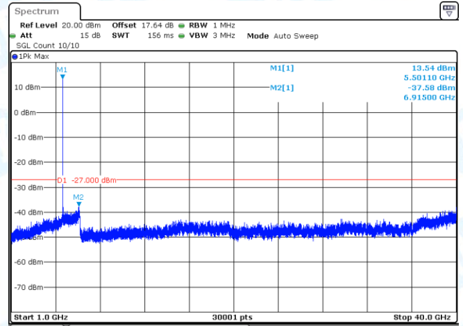
11AC20-CDD-Ant2-5500-1000~40000-PASS
