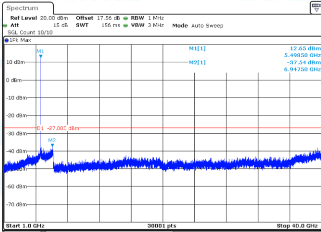
11AC20-CDD-Ant1-5500-1000~40000-PASS
