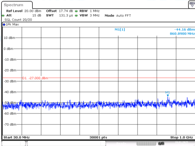
11AC20-CDD-Ant1-5825-30~1000-PASS
