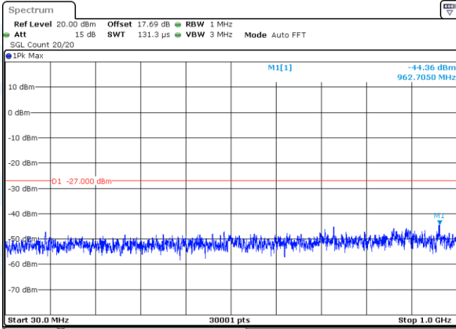
11AC40-CDD-Ant1-5795-30~1000-PASS
