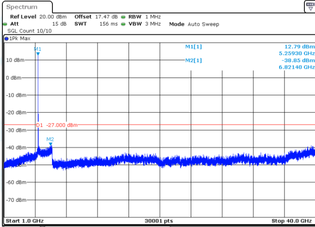
11AC20-CDD-Ant1-5260-1000~40000-PASS
