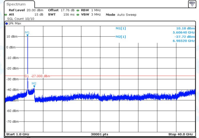
11AC80-CDD-Ant2-5610-1000~40000-PASS
