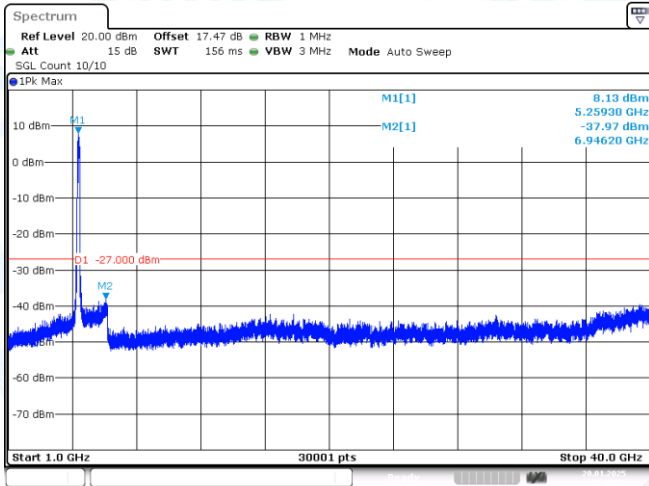
11AC160-CDD-Ant1-5250-1000~40000-PASS
