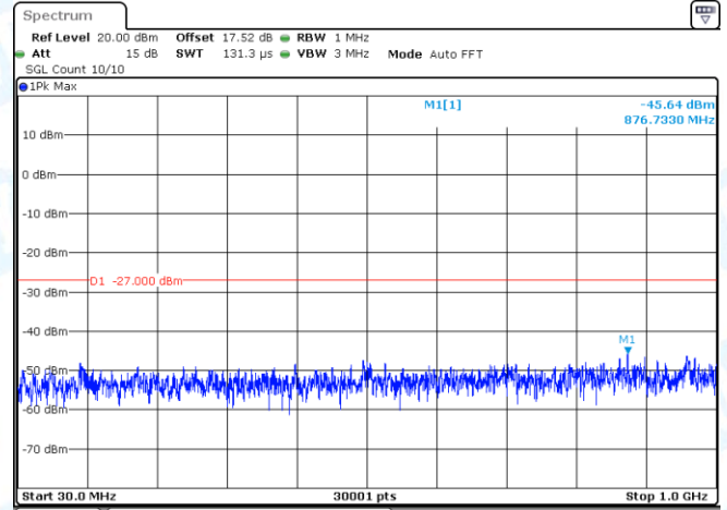
11AC40-CDD-Ant2-5270-30~1000-PASS
