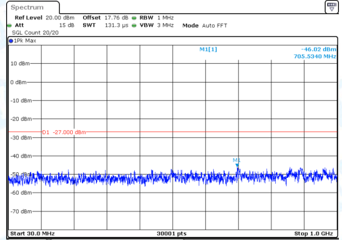
11AC80-CDD-Ant2-5775-30~1000-PASS
