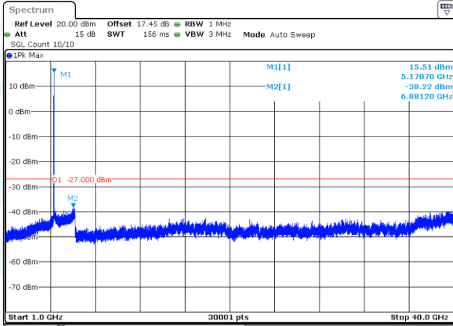
11AC20-CDD-Ant1-5180-1000~40000-PASS
