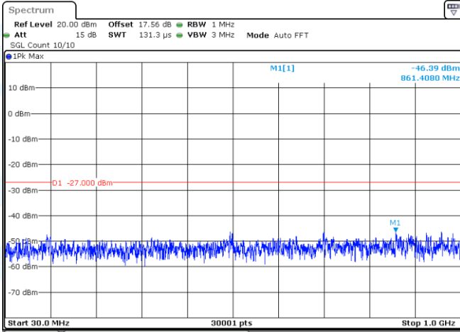
11AC80-CDD-Ant1-5530-30~1000-PASS
