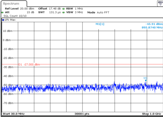
11AC20-CDD-Ant1-5240-30~1000-PASS
