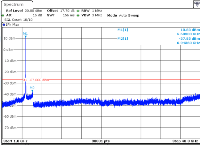
11AC80-CDD-Ant1-5610-1000~40000-PASS
