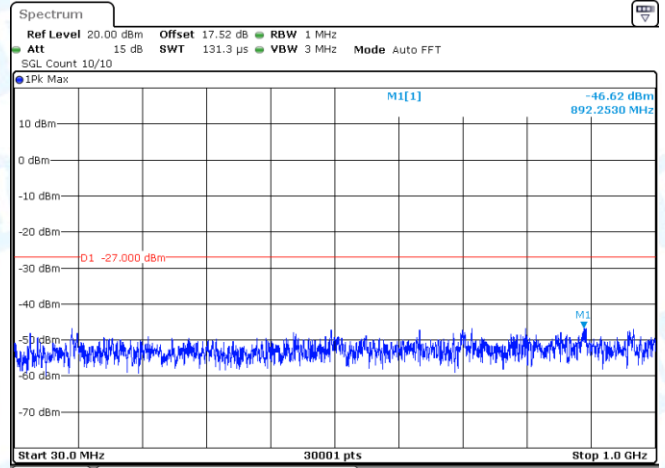
11AC20-CDD-Ant2-5320-30~1000-PASS
