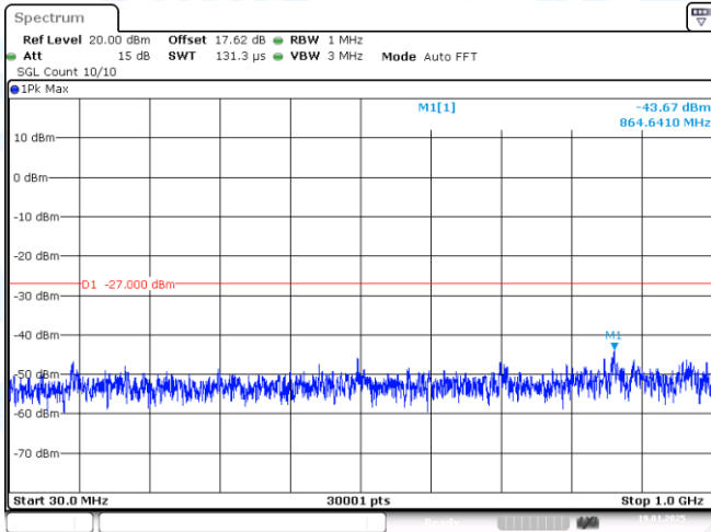
11N40-CDD-Ant1-5550-30~1000-PASS
