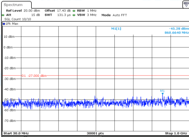
11A-CDD-Ant1-5320-30~1000-PASS
