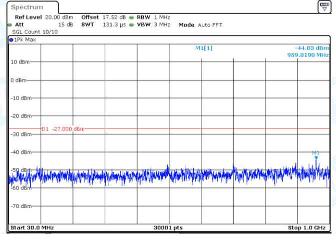
11N20-CDD-Ant2-5320-30~1000-PASS
