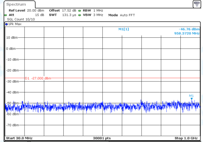
11N40-CDD-Ant2-5270-30~1000-PASS
