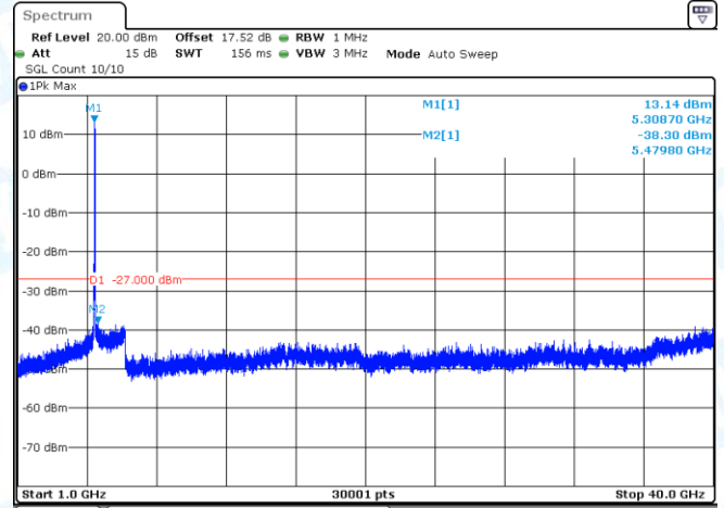
11N40-CDD-Ant2-5310-1000~40000-PASS
