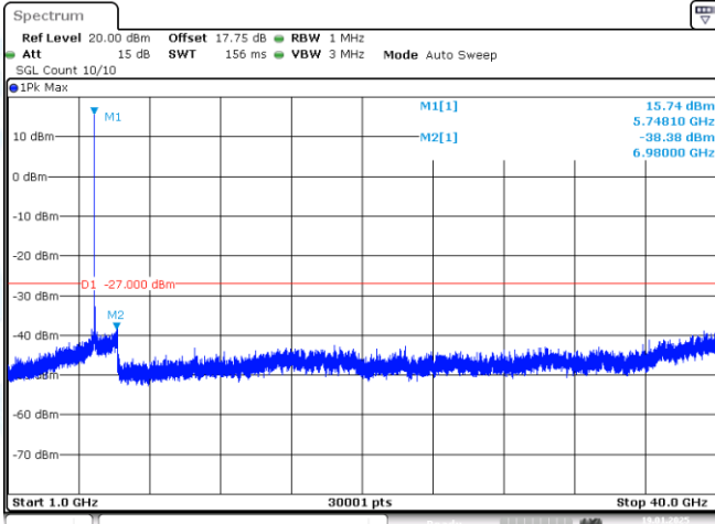
11N20-CDD-Ant1-5745-1000~40000-PASS
