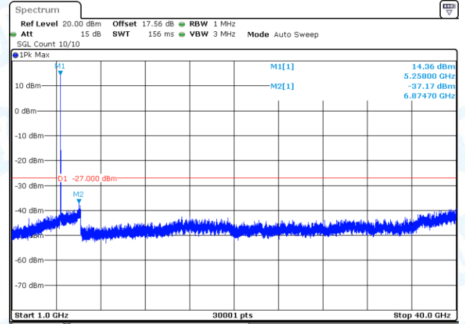
11N20-CDD-Ant2-5260-1000~40000-PASS
