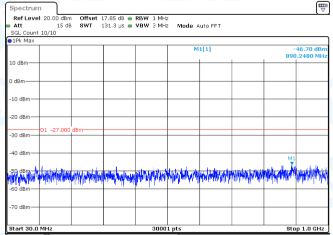
11N20-CDD-Ant2-5720-30~1000-PASS
