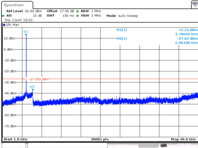
11N40-CDD-Ant1-5710-1000~40000-PASS
