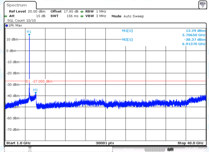
11N40-CDD-Ant2-5710-1000~40000-PASS
