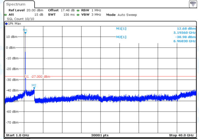
11N40-CDD-Ant2-5190-1000~40000-PASS
