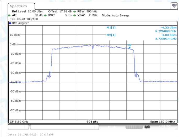
11AX80-CDD-Ant2-5690_UNII-3-PASS
