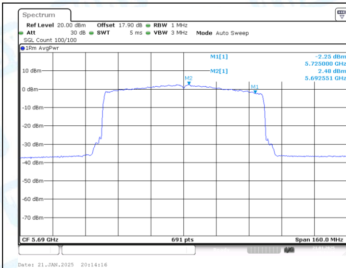
11AX80-CDD-Ant1-5690_UNII-2C-PASS
