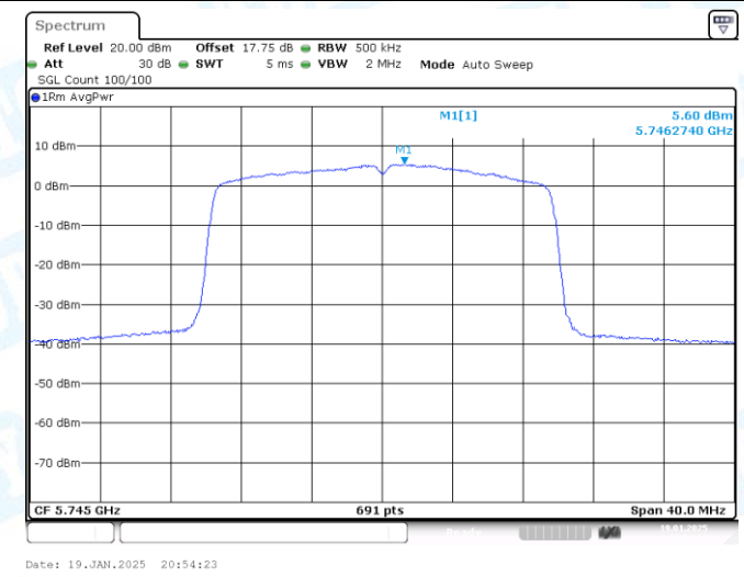
11AX20-CDD-Ant2-5745-PASS
