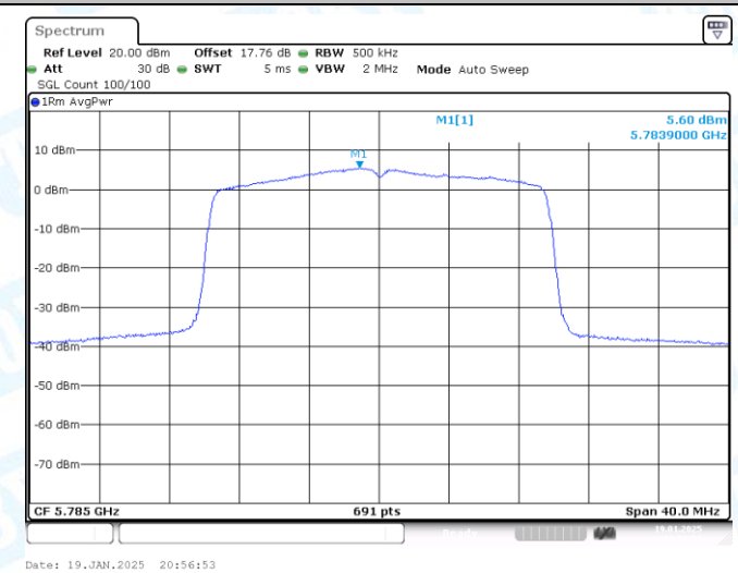
11AX20-CDD-Ant2-5785-PASS
