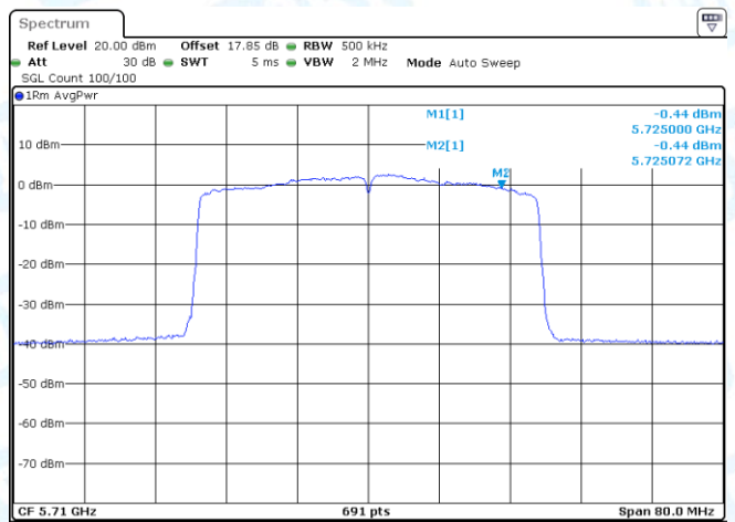
11AX40-CDD-Ant2-5710_UNII-2C-PASS
