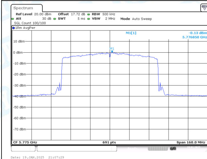
11AX80-CDD-Ant1-5775-PASS
