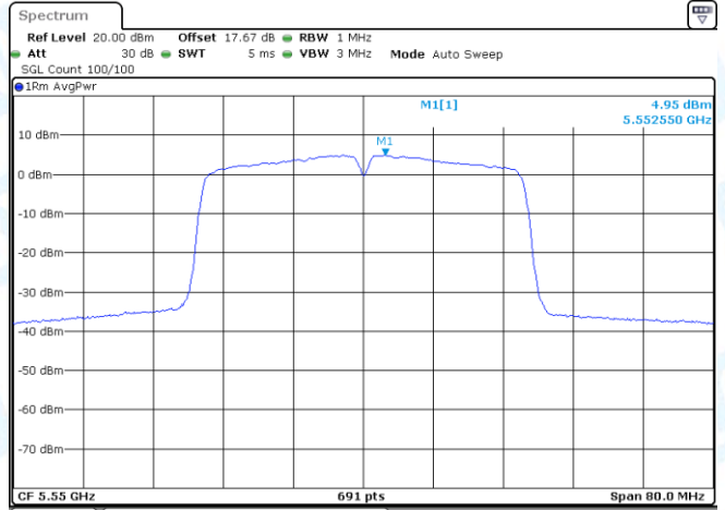
11AC40-CDD-Ant2-5550-PASS
