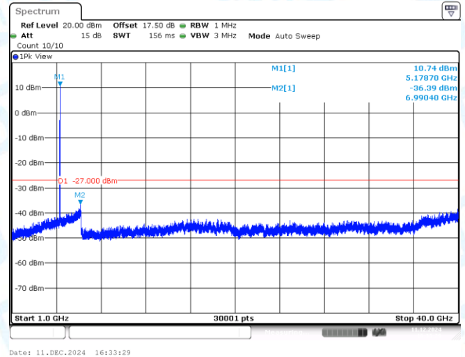
11A-Ant2-5180-1000~40000-PASS
