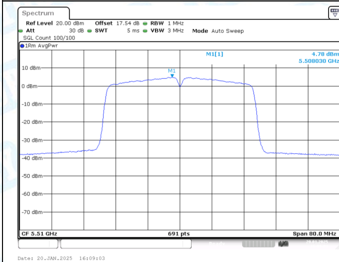
11AC40-CDD-Ant1-5510-PASS
