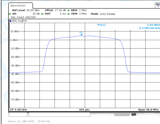
11AX20-CDD-Ant1-5280-PASS
