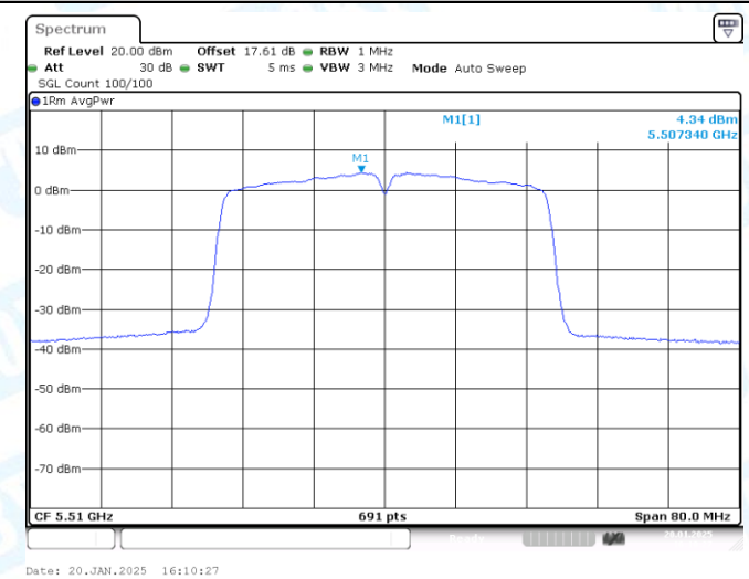
11AC40-CDD-Ant2-5510-PASS
