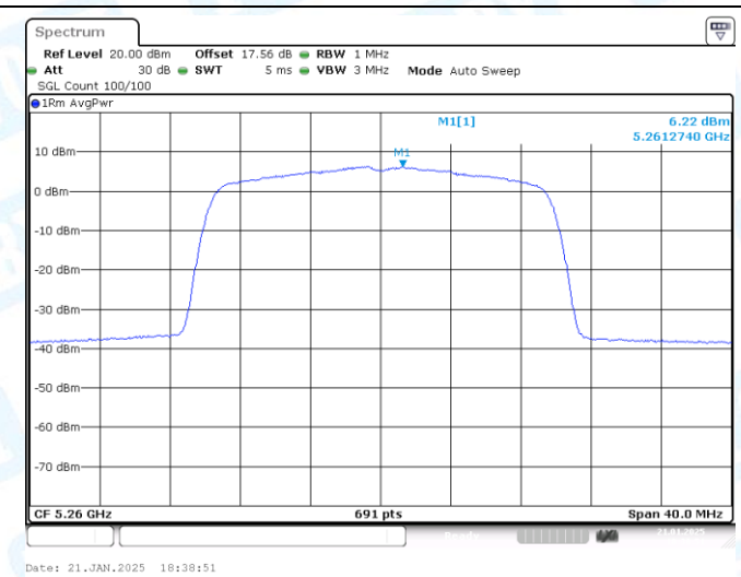
11AX20-CDD-Ant2-5260-PASS
