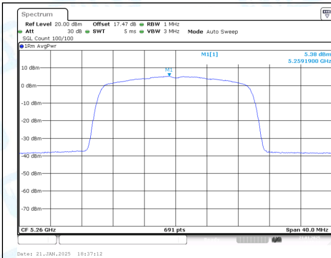
11AX20-CDD-Ant1-5260-PASS
