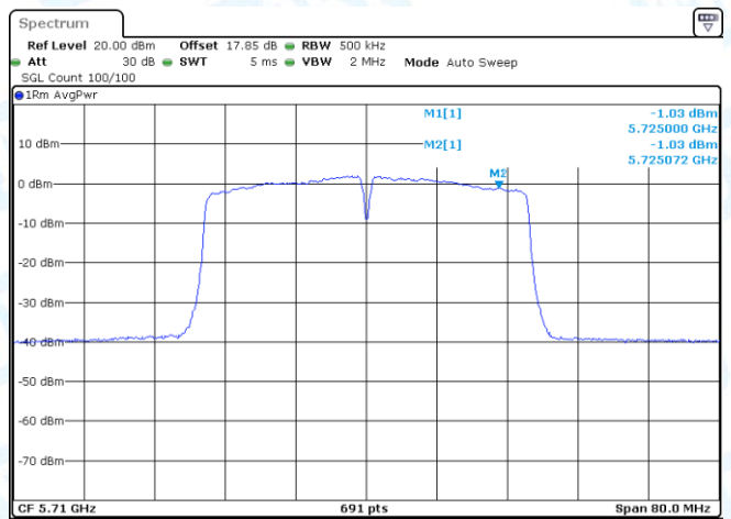
11AC40-CDD-Ant2-5710_UNII-2C-PASS
