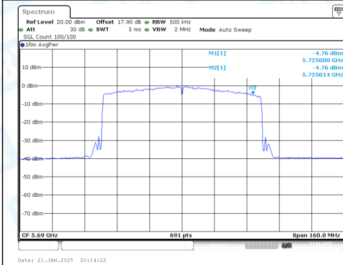
11AX80-CDD-Ant1-5690_UNII-3-PASS
