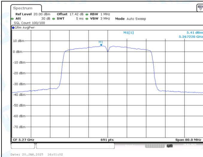
11AC40-CDD-Ant1-5270-PASS
