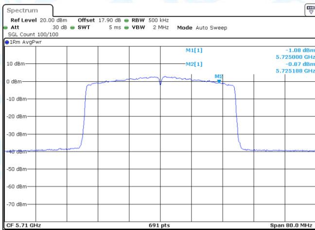
11AX40-CDD-Ant1-5710_UNII-2C-PASS
