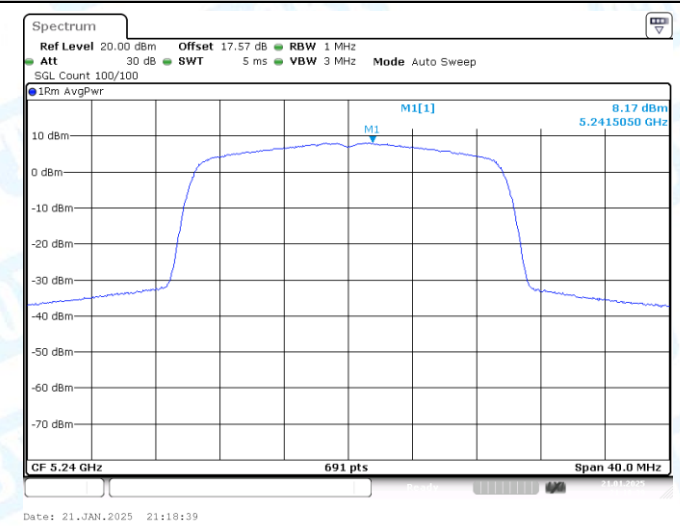
11AX20-CDD-Ant2-5240-PASS
