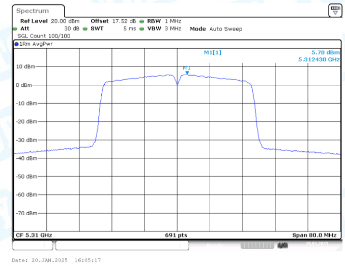
11AC40-CDD-Ant2-5310-PASS
