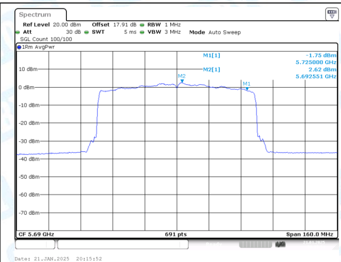
11AX80-CDD-Ant2-5690_UNII-2C-PASS
