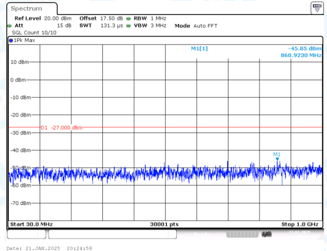
11A-CDD-Ant2-5180-30~1000-PASS
