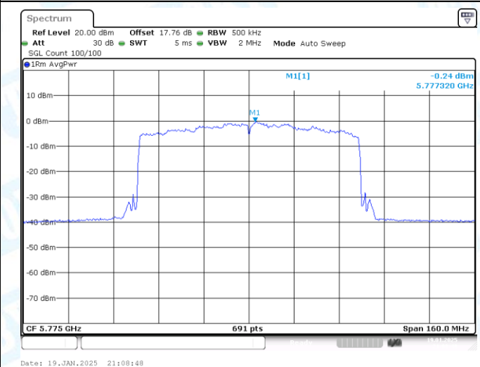
11AX80-CDD-Ant2-5775-PASS
