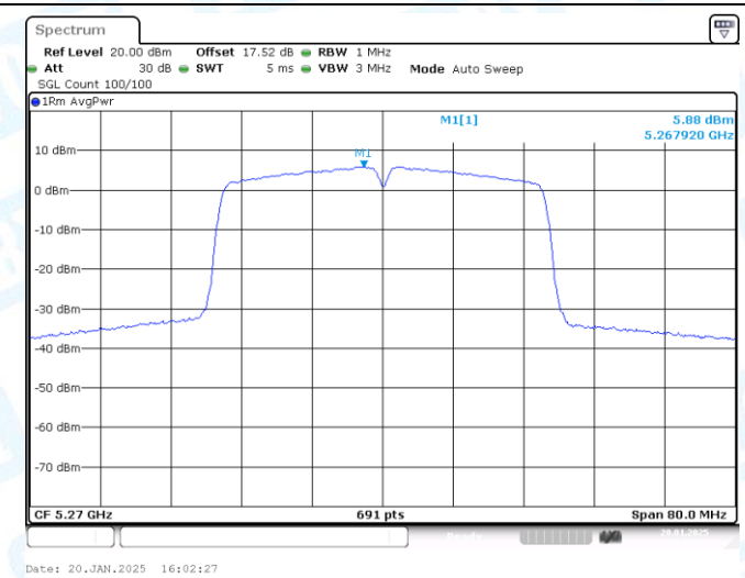
11AC40-CDD-Ant2-5270-PASS
