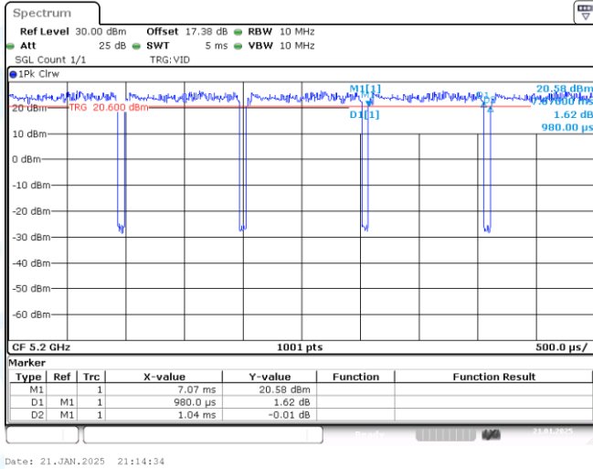
NTNV-11AX20-CDD-Ant1-5200
