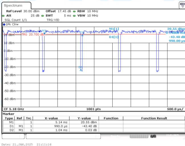
NTNV-11AX20-CDD-Ant1-5180
