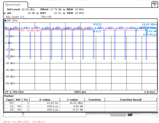
NTNV-11AC40-CDD-Ant2-5795
