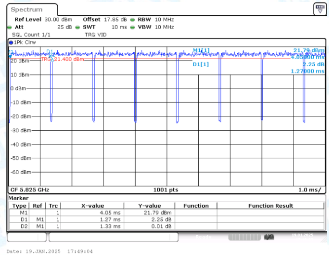
NTNV-11AC20-CDD-Ant2-5825
