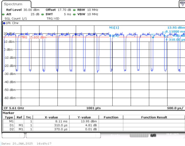
NTNV-11AC80-CDD-Ant1-5610
