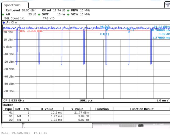
NTNV-11AC20-CDD-Ant1-5825
