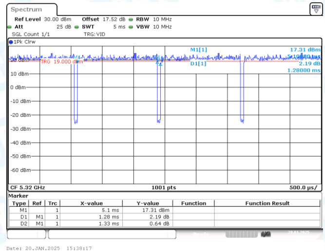
NTNV-11AC20-CDD-Ant2-5320
