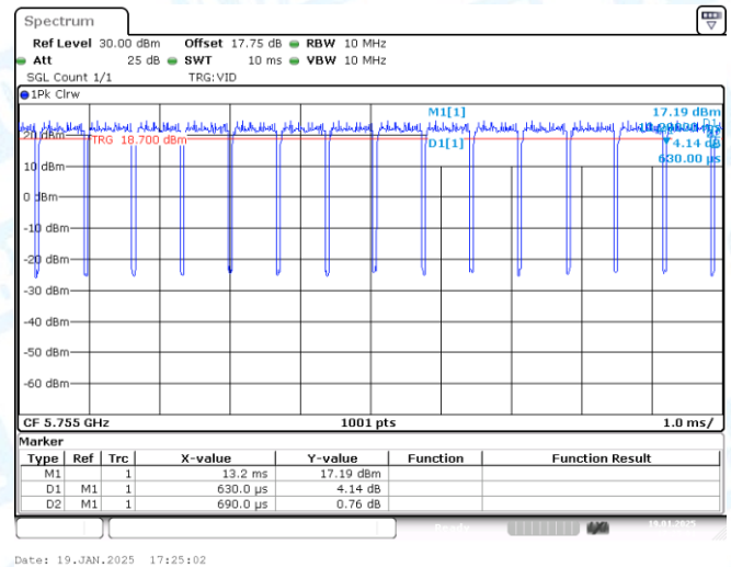
NTNV-11N40-CDD-Ant2-5755
