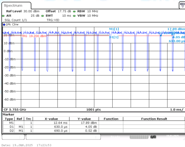
NTNV-11N40-CDD-Ant1-5755
