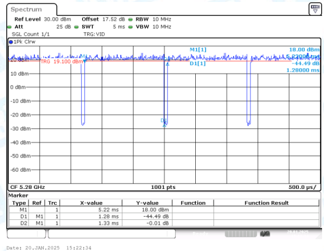
NTNV-11AC20-CDD-Ant2-5280
