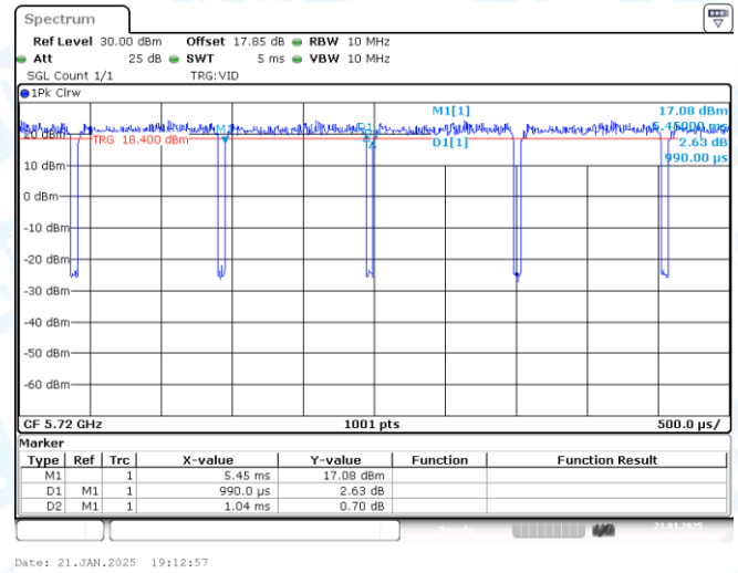
NTNV-11AX20-CDD-Ant2-5720
