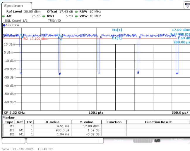
NTNV-11AX20-CDD-Ant1-5320
