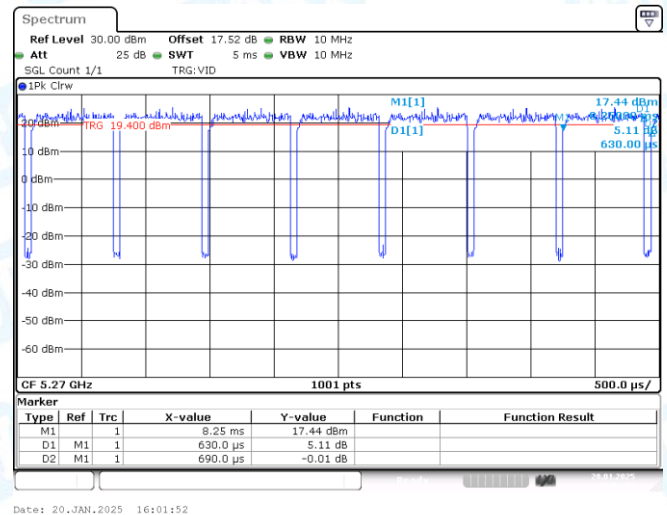
NTNV-11AC40-CDD-Ant2-5270
