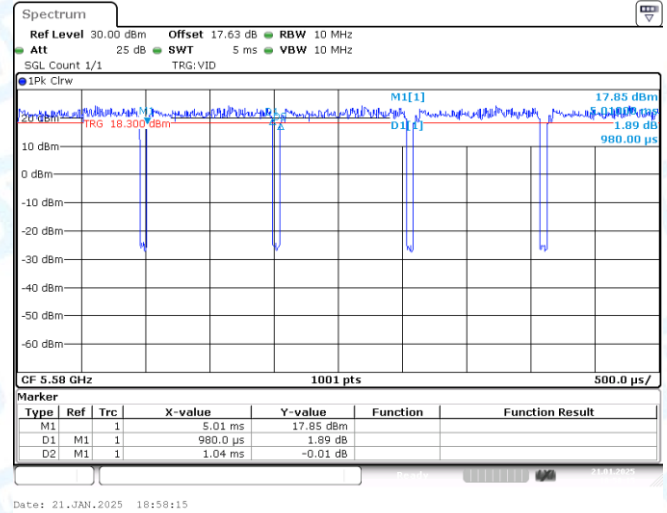
NTNV-11AX20-CDD-Ant2-5580
