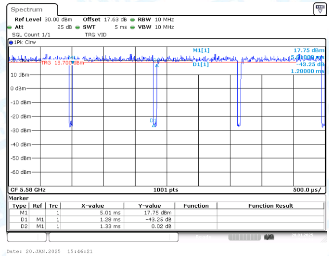
NTNV-11AC20-CDD-Ant2-5580
