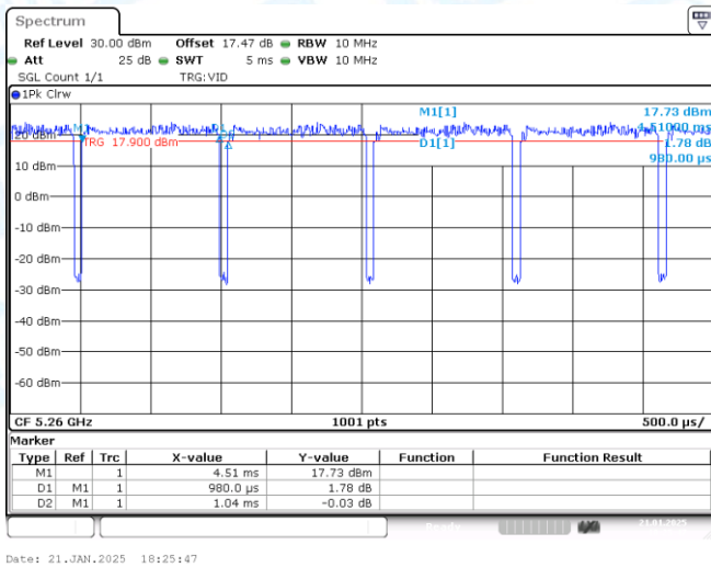
NTNV-11AX20-CDD-Ant1-5260
