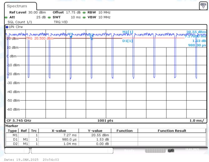
NTNV-11AX20-CDD-Ant2-5745
