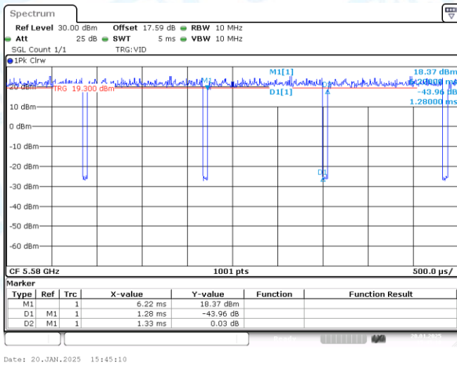
NTNV-11AC20-CDD-Ant1-5580
