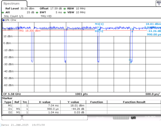
NTNV-11AX20-CDD-Ant1-5580
