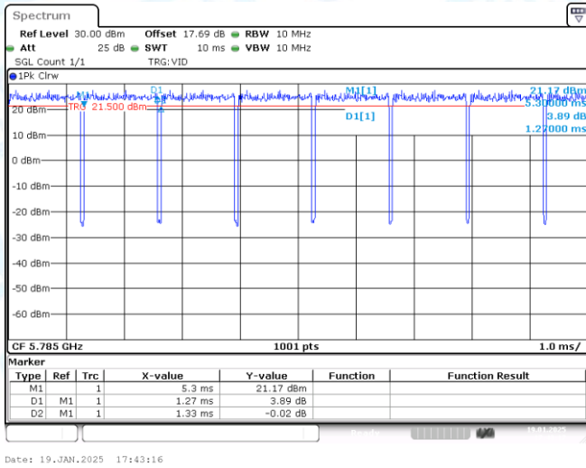
NTNV-11AC20-CDD-Ant1-5785
