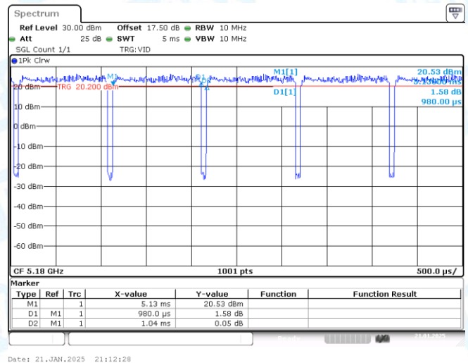
NTNV-11AX20-CDD-Ant2-5180
