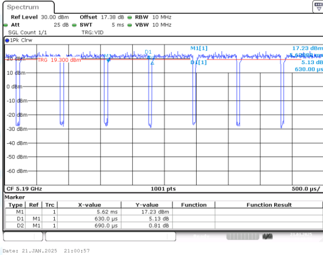
NTNV-11AC40-CDD-Ant1-5190
