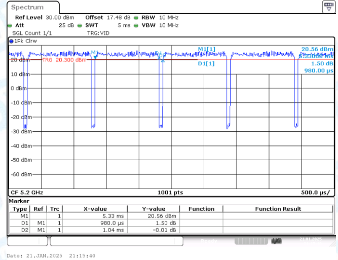
NTNV-11AX20-CDD-Ant2-5200
