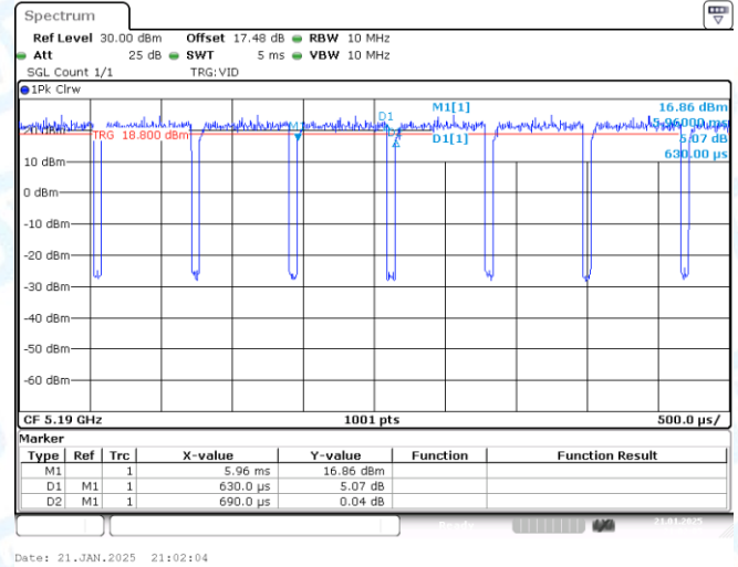
NTNV-11AC40-CDD-Ant2-5190
