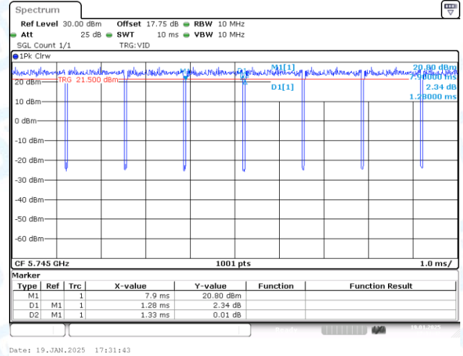
NTNV-11AC20-CDD-Ant2-5745
