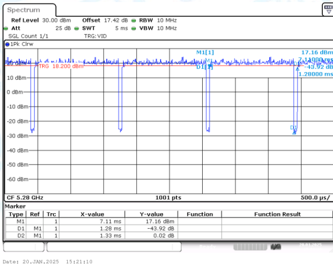
NTNV-11AC20-CDD-Ant1-5280
