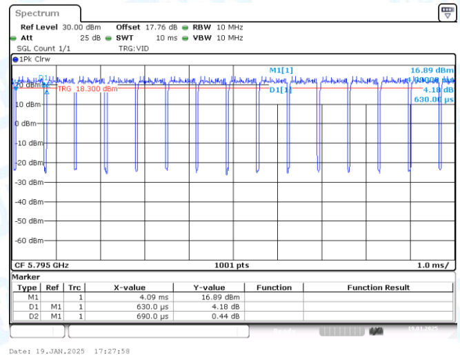
NTNV-11N40-CDD-Ant2-5795
