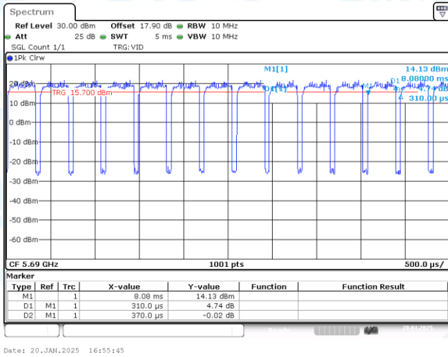
NTNV-11AC80-CDD-Ant1-5690
