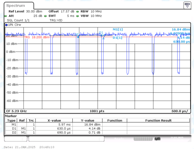
NTNV-11N40-CDD-Ant2-5230
