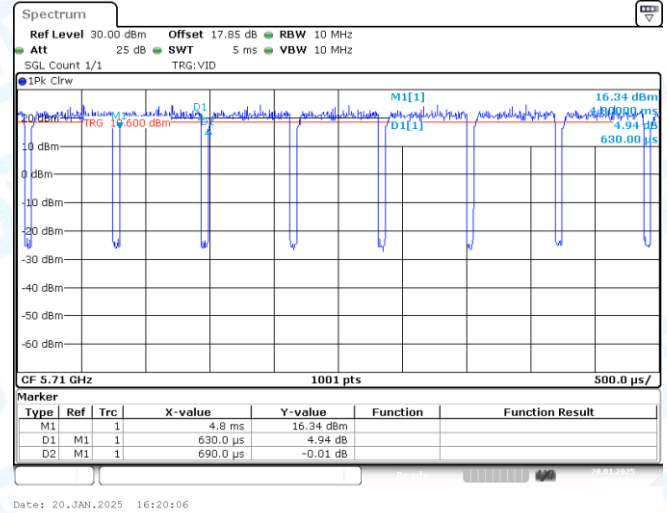
NTNV-11AC40-CDD-Ant2-5710
