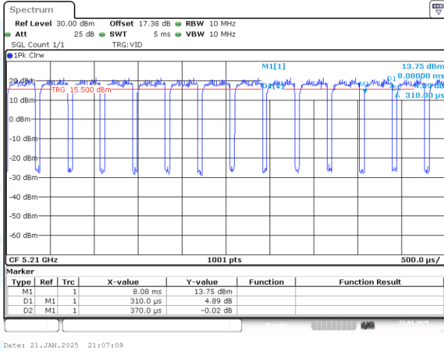
NTNV-11AC80-CDD-Ant1-5210
