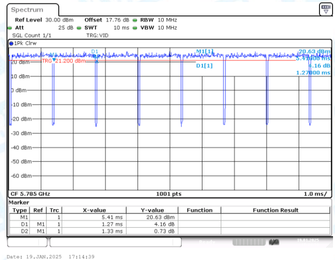
NTNV-11N20-CDD-Ant2-5785
