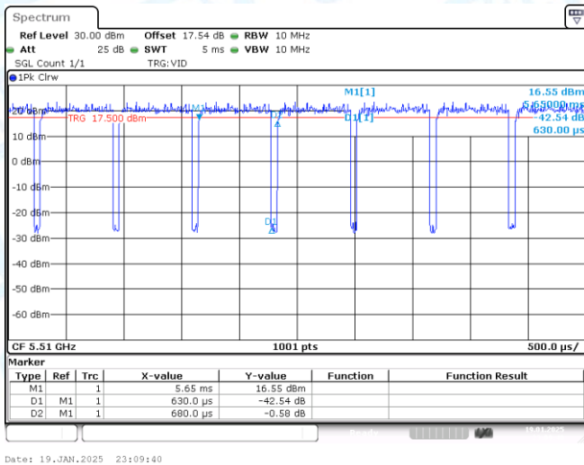
NTNV-11N40-CDD-Ant1-5510
