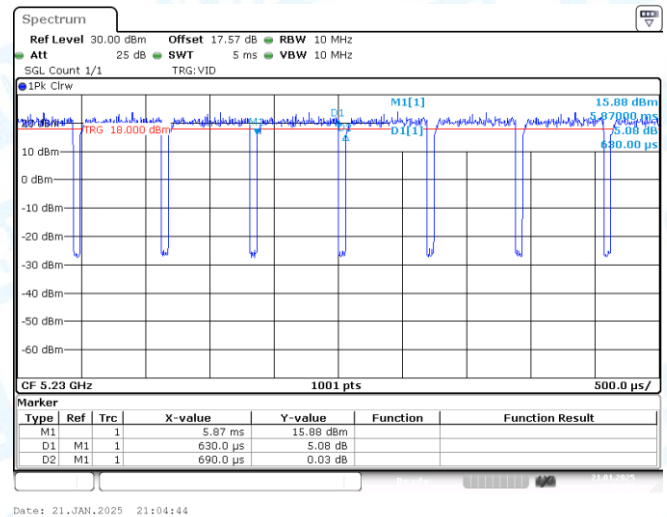
NTNV-11AC40-CDD-Ant2-5230
