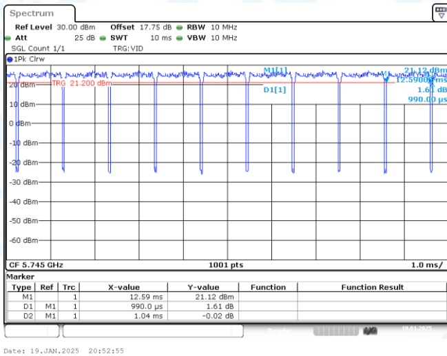
NTNV-11AX20-CDD-Ant1-5745
