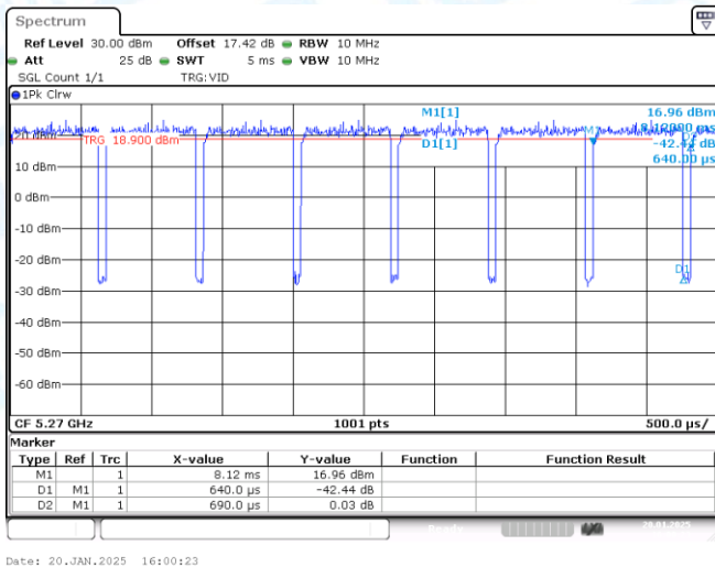
NTNV-11AC40-CDD-Ant1-5270
