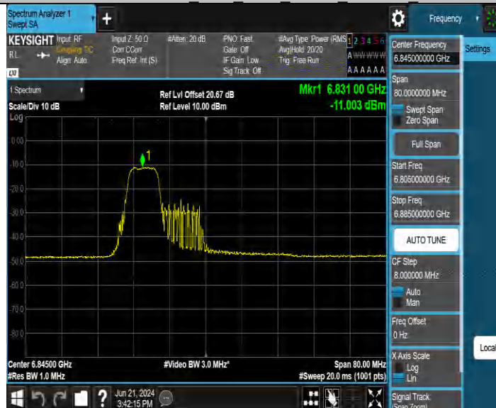
11BE40MIMO Ant3 6845 52+26 OFDMA 1
