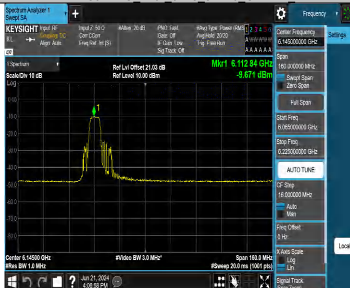
11BE80MIMO Ant2 6145 52+26 OFDMA 1
