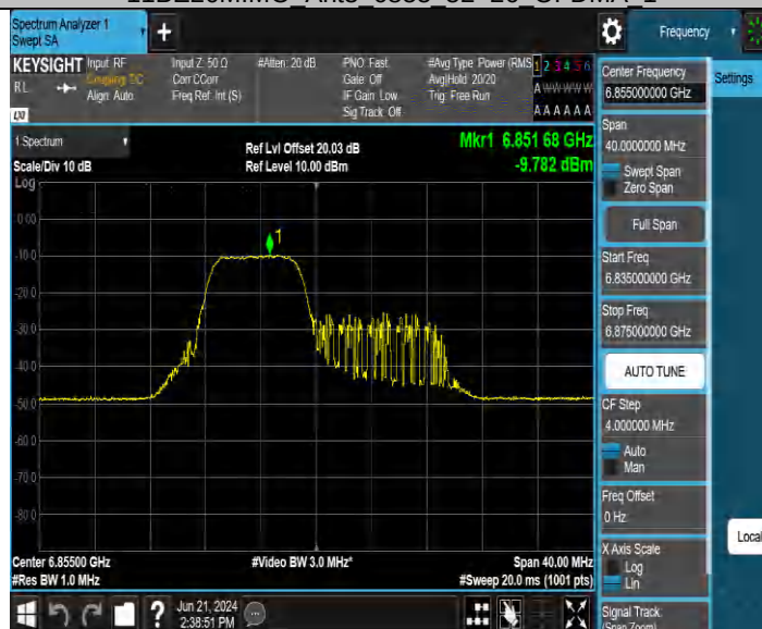
11BE20MIMO Ant4 6855 52+26 OFDMA 1
