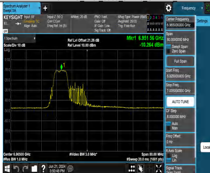
11BE40MIMO Ant2 6965 52+26 OFDMA 1
