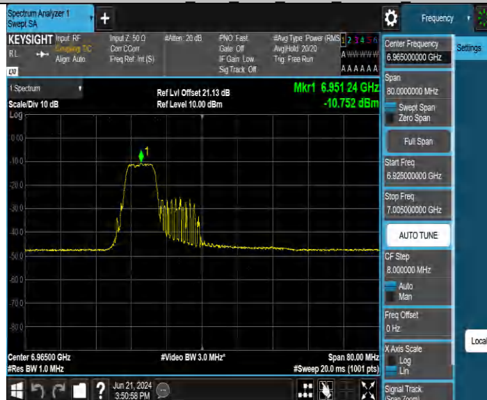
11BE40MIMO Ant3 6965 52+26 OFDMA 1
