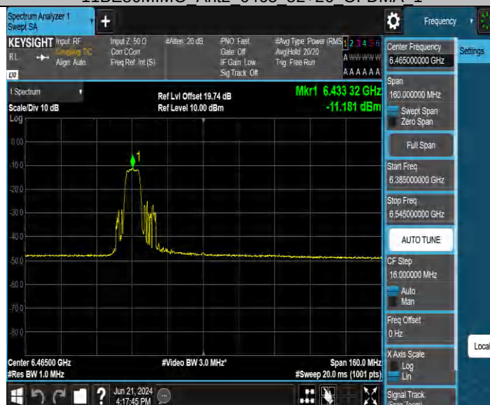
11BE80MIMO Ant3 6465 52+26 OFDMA 1
