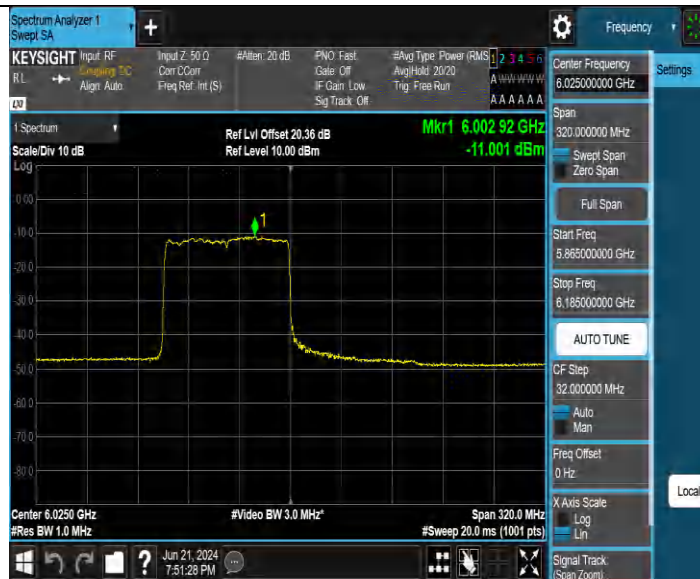
11BE160MIMO Ant3 6025 996Tone RU67
