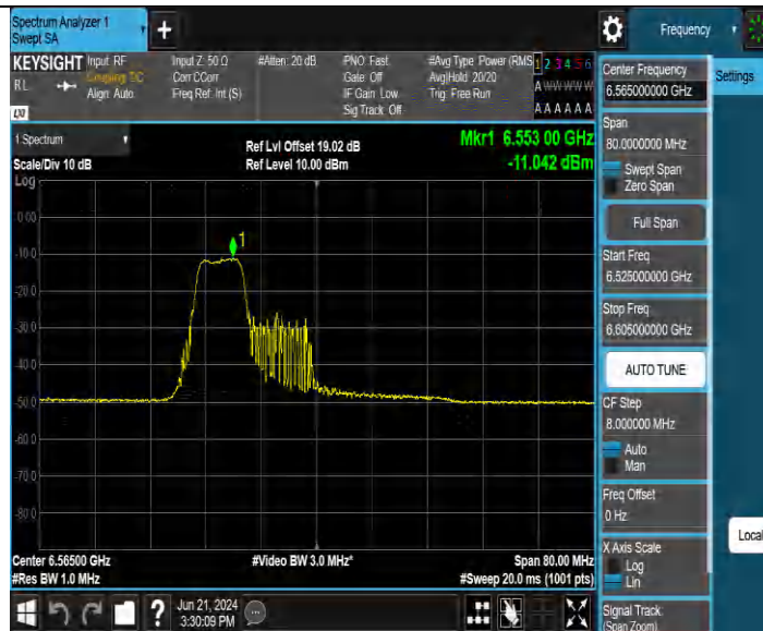
11BE40MIMO Ant3 6565 52+26 OFDMA 1
