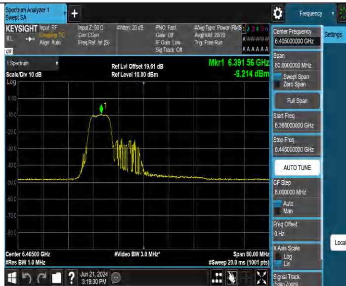
11BE40MIMO Ant4 6405 52+26 OFDMA 1
