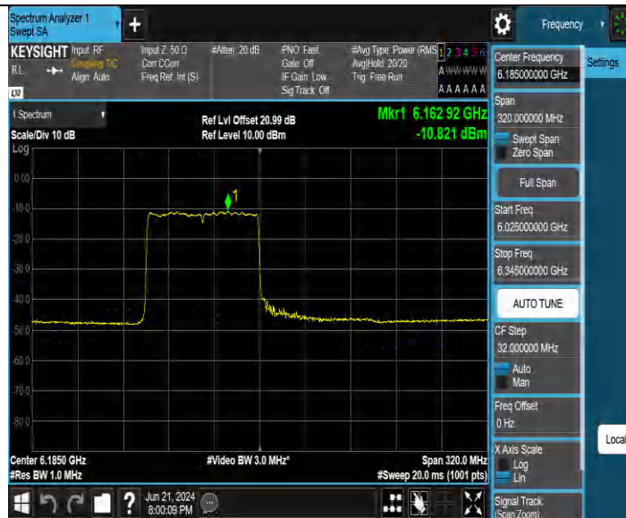
11BE160MIMO Ant2 6185_996Tone RU67
