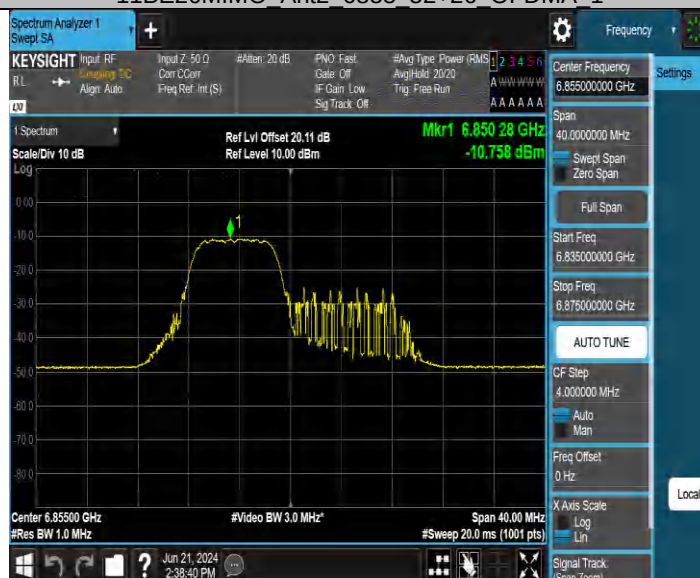
11BE20MIMO Ant3 6855 52+26 OFDMA 1
