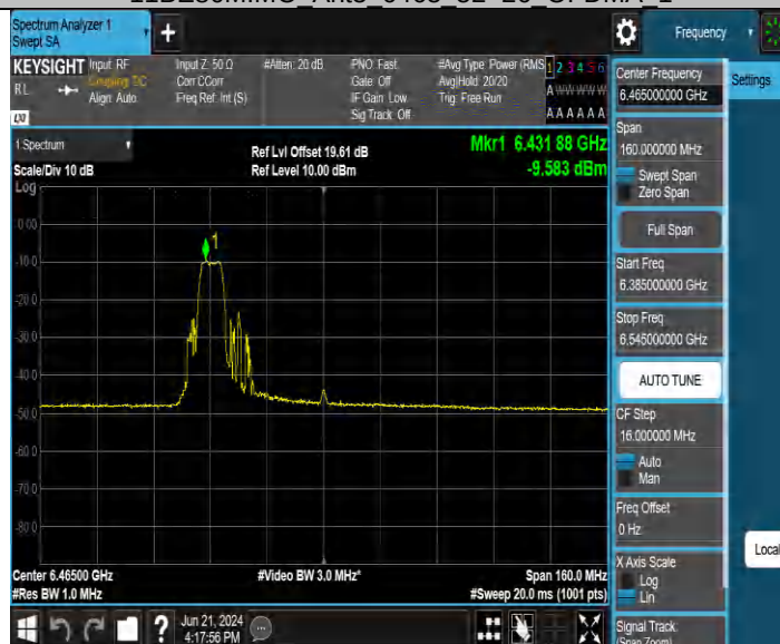
11BE80MIMO Ant4 6465 52+26 OFDMA 1
