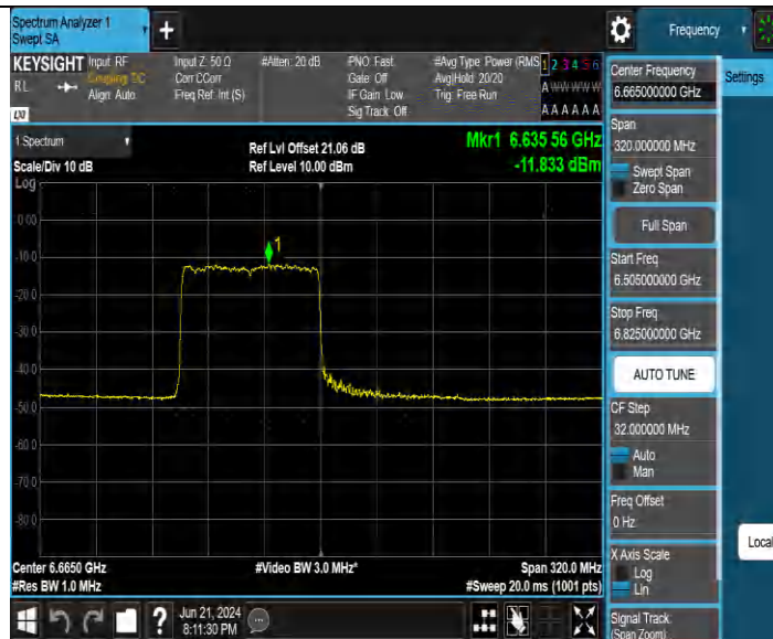
11BE160MIMO Ant2 6665 996Tone RU67
