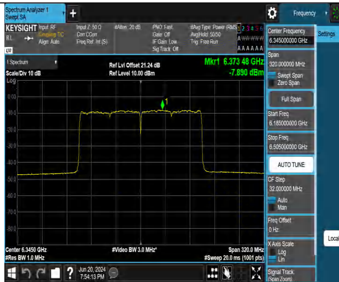
11BE160MIMO Ant2 6345
