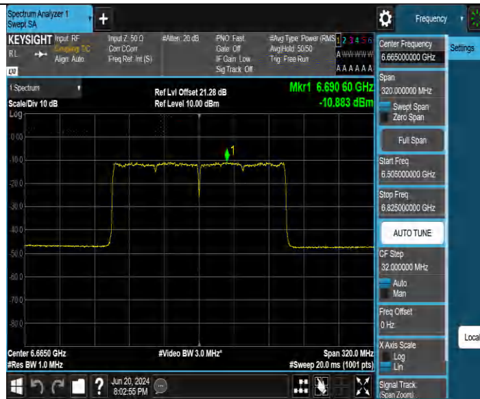
11BE160MIMO Ant3 6665
