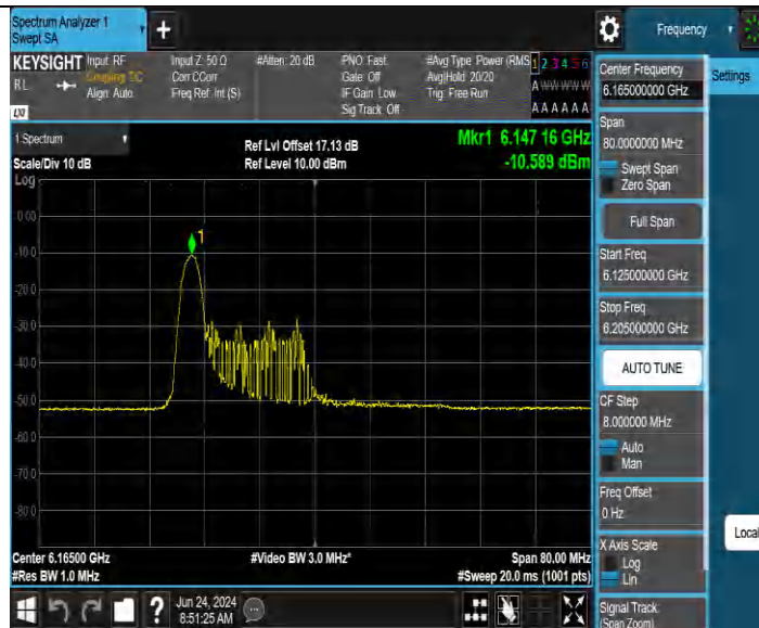
11BE40MIMO_Ant2_6165_26Tone_RU0
