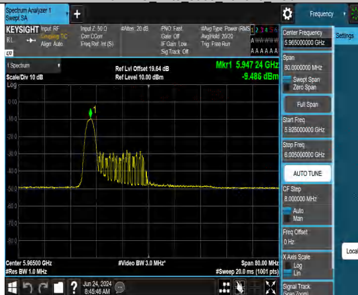
11BE40MIMO_Ant4_5965_26Tone_RU0
