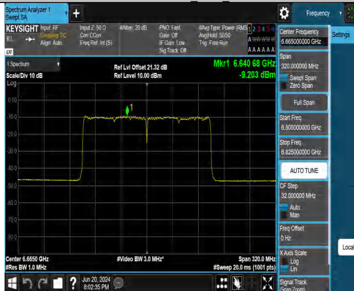
11BE160MIMO Ant2 6665
