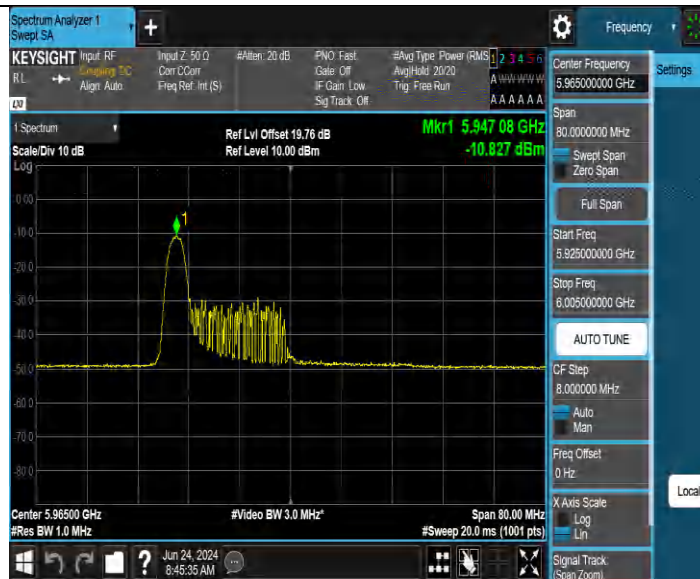
11BE40MIMO_Ant3_5965_26Tone_RU0
