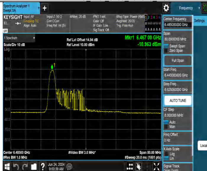
11BE40MIMO_Ant3_6485_26Tone_RU0
