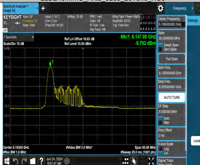
11BE40MIMO_Ant4_6165_26Tone_RU0
