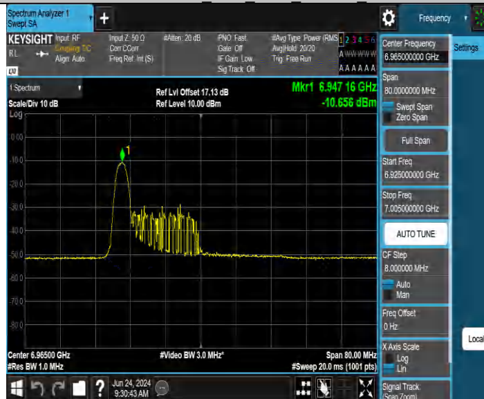
11BE40MIMO_Ant3_6965_26Tone_RU0
