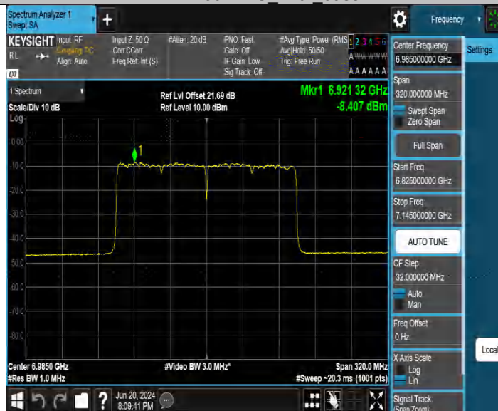
11BE160MIMO Ant2 6985
