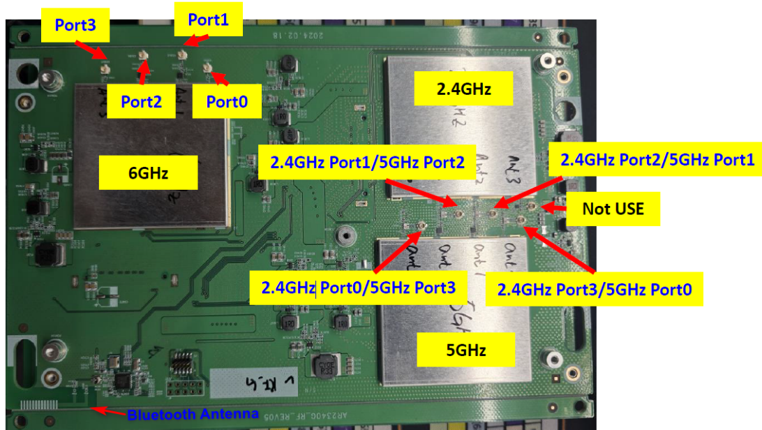
View 15#(Antenna Location)
