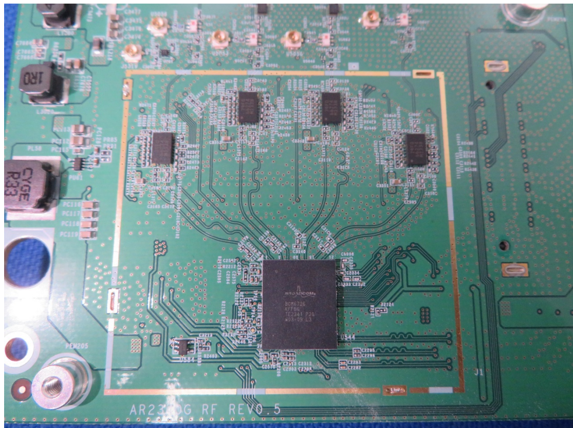
View 13#(2.4GHz Wi-Fi Chip)
