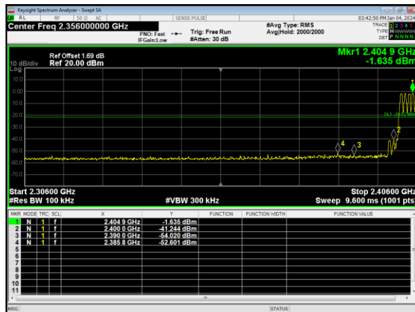
Band-edge Emission
