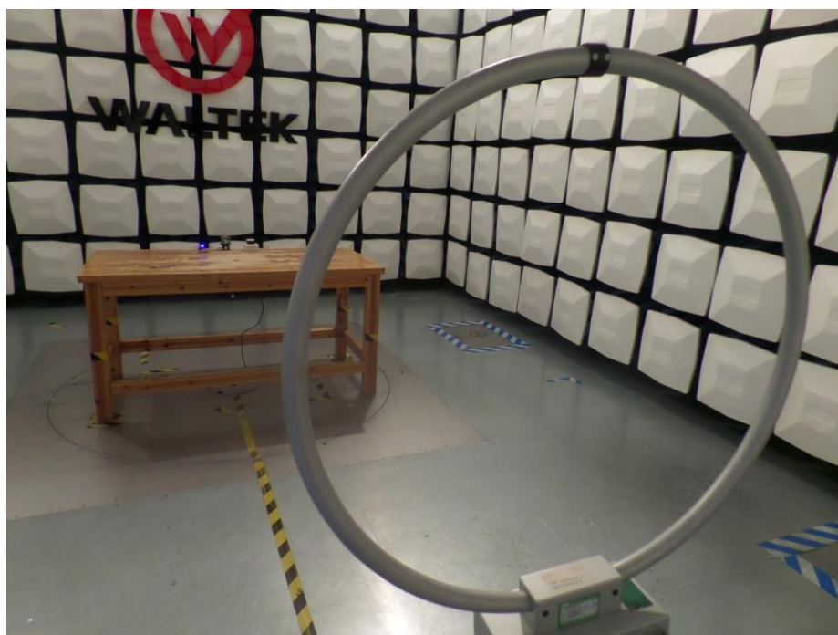
Test Setup For Radiated Emission (9kHz to 30MHz)
