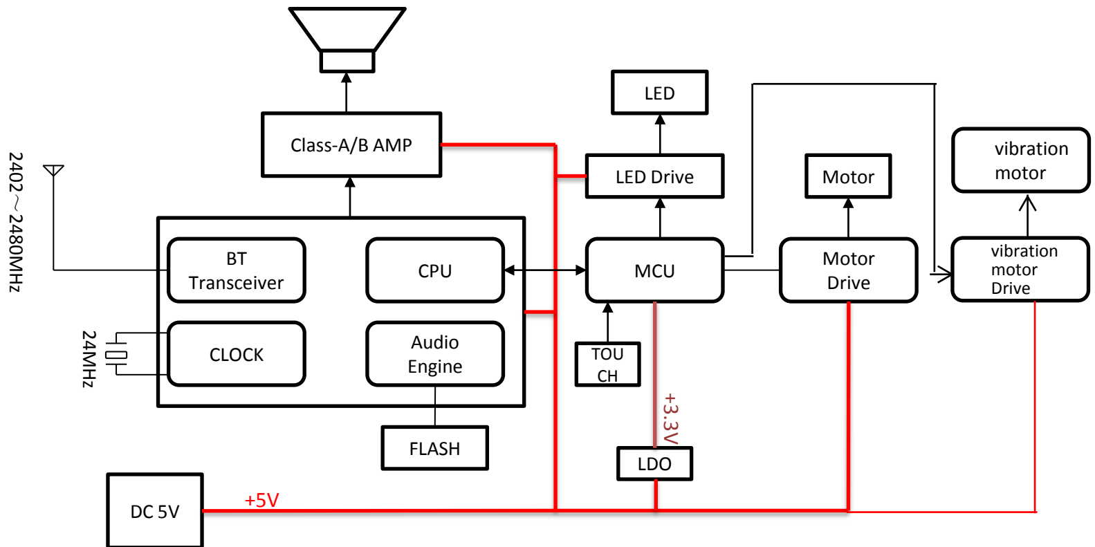
Swing 1.5 MCK Block Diagram
