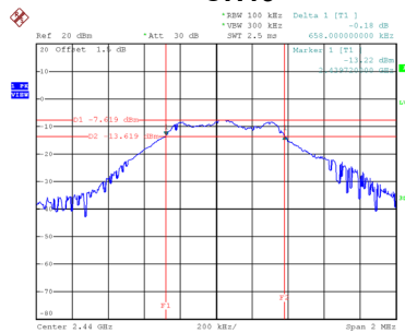
6dB Bandwidth CH19
