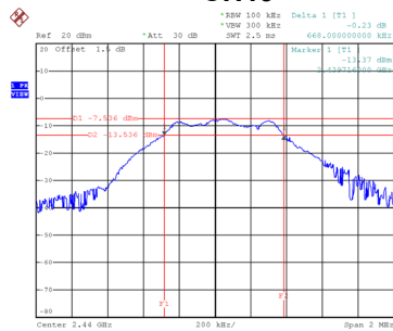
6dB Bandwidth CH19
