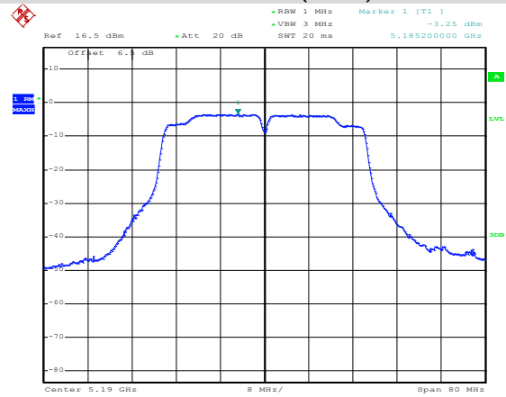
ANT2 802.11n(HT40)
