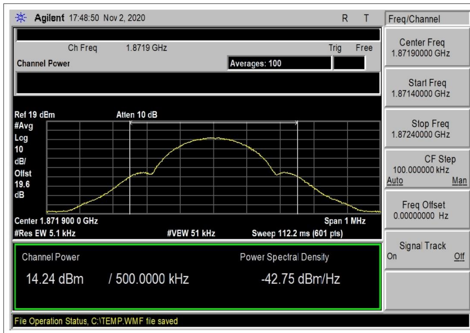
UL 1850-1915 AGC+3d
