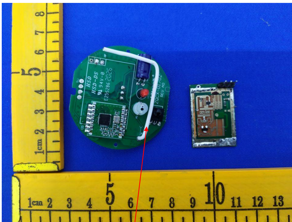
915MHz Antenna
