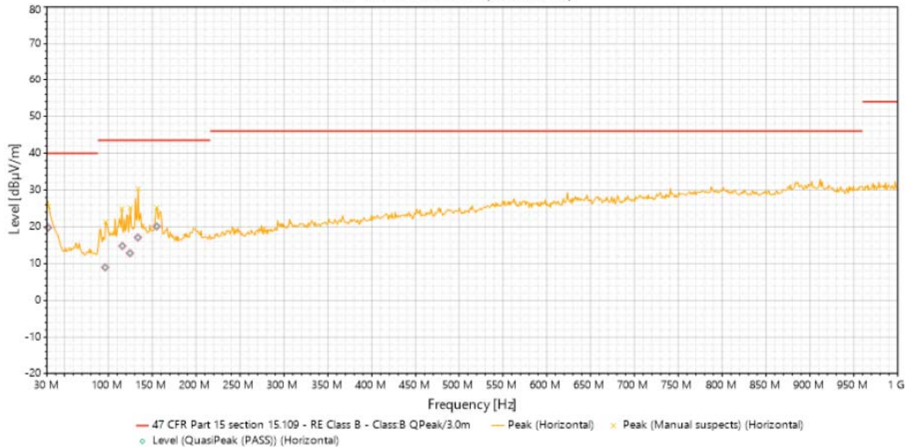
#2 - 30MHz-1GHz (Horizontal)
