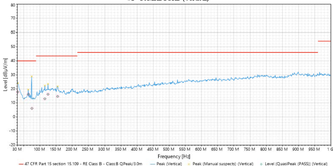
#1 - 30MHz-1GHz (Vertical)
