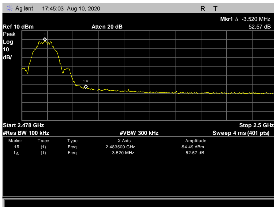
Figure 70: Conducted Band Edge, 2480 MHz
