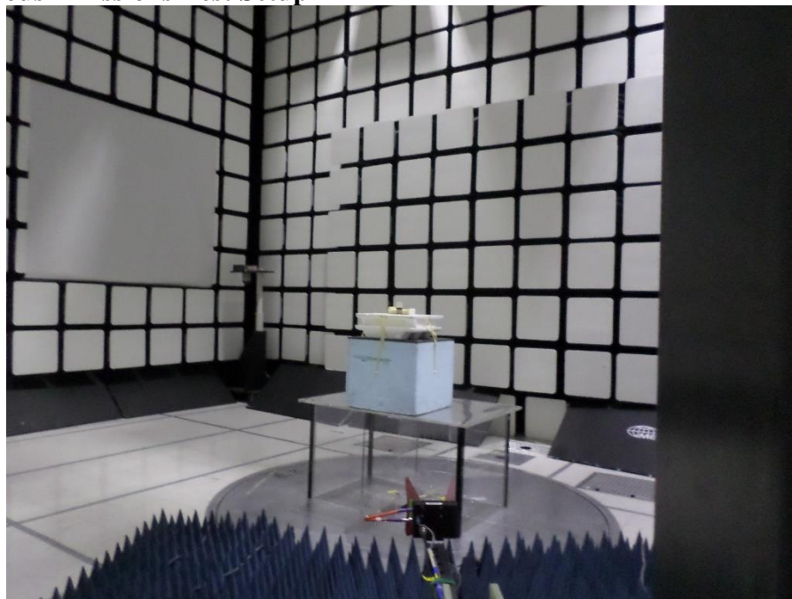
Figure 56: Radiated Emissions, 1-18 GHz - Setup Antenna View
