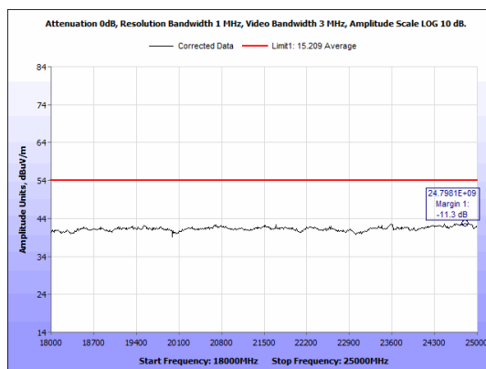
Figure 43: Radiated Emissions, 2480 MHz - 18-25 GHz - Average - Horizontal.
