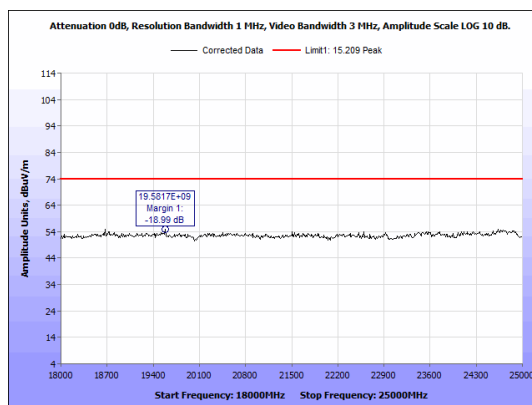
Figure 21: Radiated Emissions, 2402 MHz - 18-25 GHz - Peak - Horizontal.
