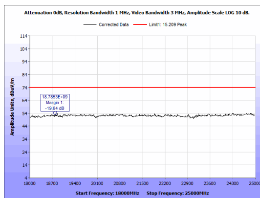
Figure 45: Radiated Emissions, 2480 MHz - 18-25 GHz - Peak - Horizontal.
