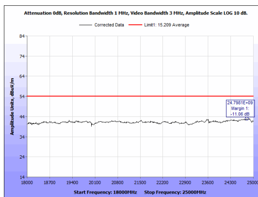
Figure 44: Radiated Emissions, 2480 MHz - 18-25 GHz - Average - Vertical.
