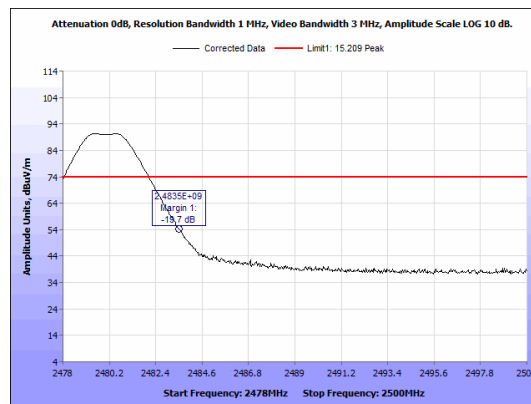
Figure 55: Radiated Band Edge, 2480 MHz - Peak - Vertical.
