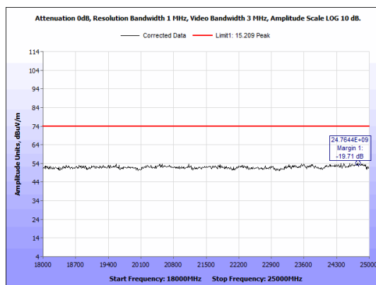
Figure 22: Radiated Emissions, 2402 MHz - 18-25 GHz - Peak - Vertical.
