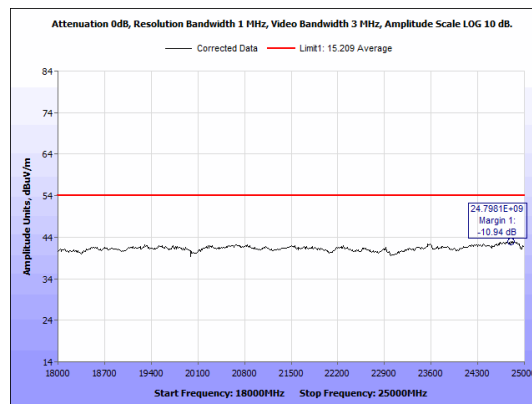
Figure 31: Radiated Emissions, 2440 MHz - 18-25 GHz - Average - Horizontal.
