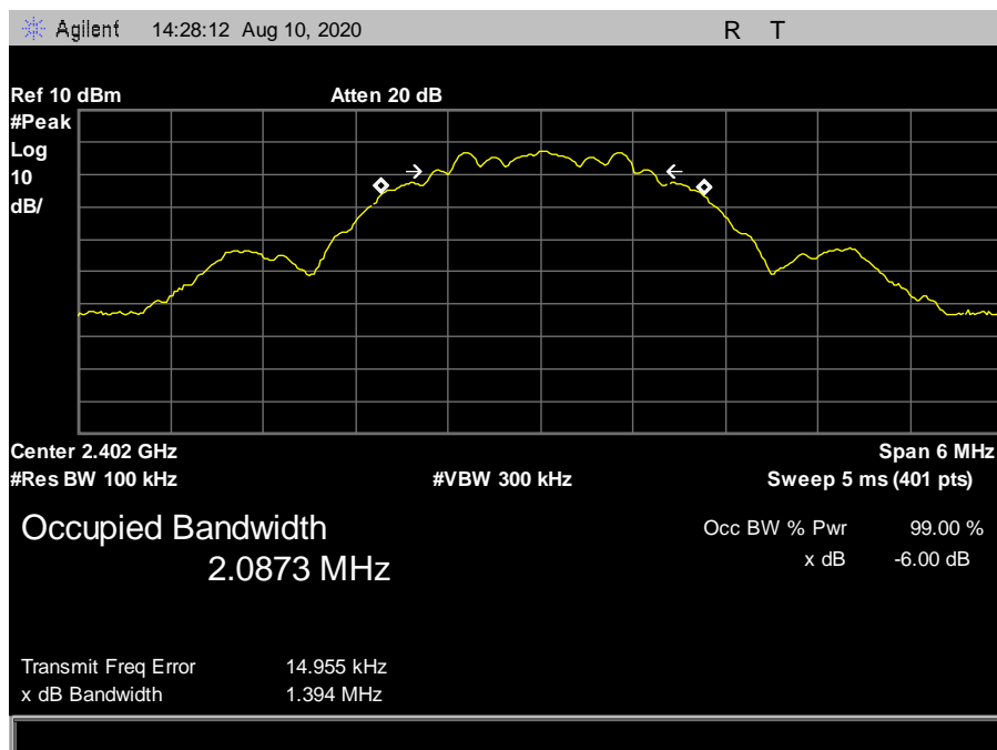
Figure 4: 6 dB Occupied Bandwidth, 2402 MHz - 1.394 MHz
