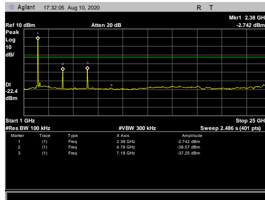
Figure 63: Conducted Spurious Emissions, 2402 MHz - 1-25 GHz
