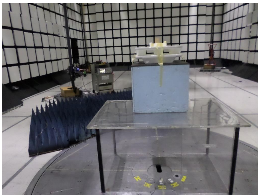
Figure 61: Radiated Emissions, 18-25 GHz - Setup Rear View
