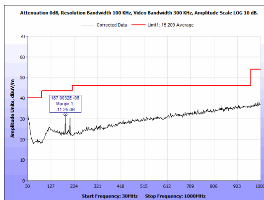
Figure 36: Radiated Emissions, 2480 MHz - 30-1000 MHz - Horizontal.
