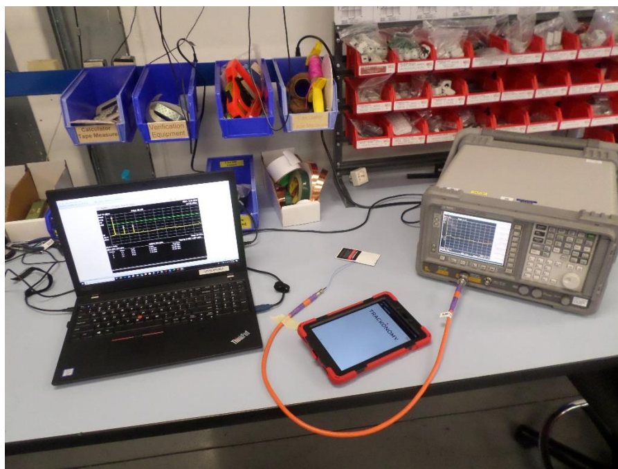
Figure 10: Conducted Measurement, Test Setup
