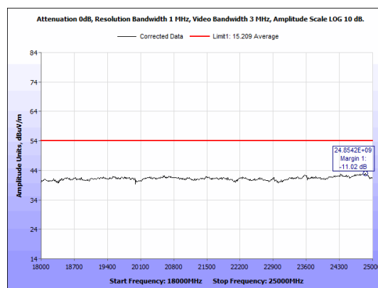
Figure 32: Radiated Emissions, 2440 MHz - 18-25 GHz - Average - Vertical.
