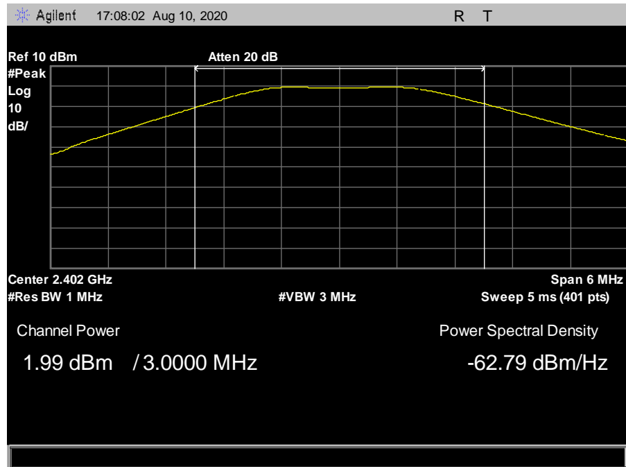
Figure 7: Conducted Output Power, 2402 MHz - (1.99 dBm)
