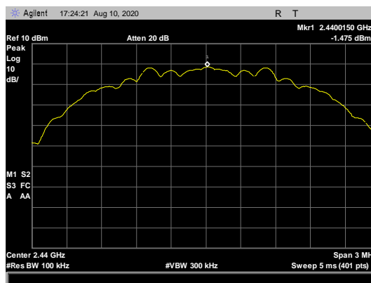
Figure 73: Power Spectral Density, 2440 MHz - (-1.475 dBm)
