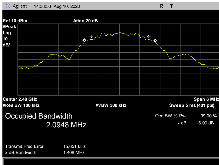
Figure 6: 6 dB Occupied Bandwidth, 2480 MHz - 1.408 MHz
