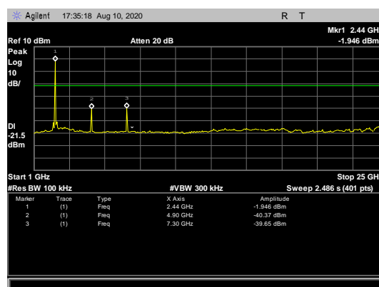
Figure 65: Conducted Spurious Emissions, 2440 MHz - 1-25 GHz
