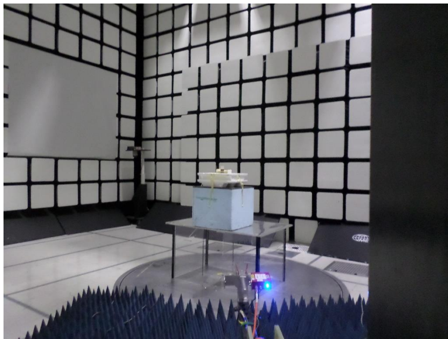
Figure 59: Radiated Emissions, 18-25 GHz - Setup Antenna View
