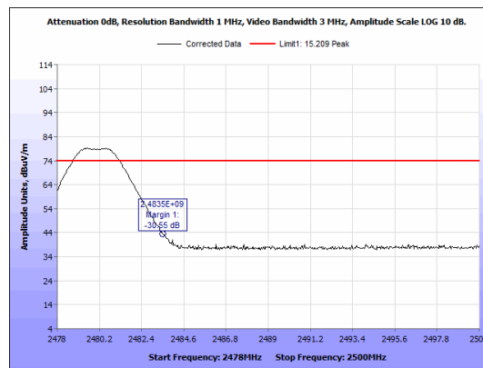
Figure 54: Radiated Band Edge, 2480 MHz - Peak - Horizontal.
