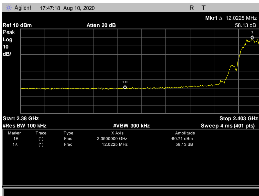
Figure 69: Conducted Band Edge, 2402 MHz
