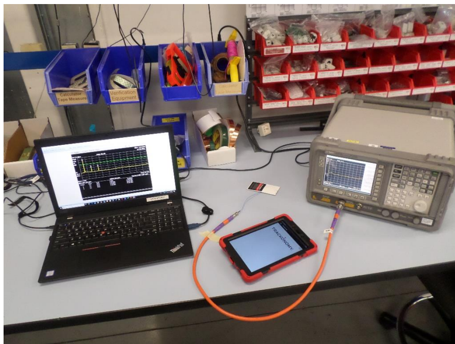
Figure 71: Conducted Spurious Emissions, Test Setup
