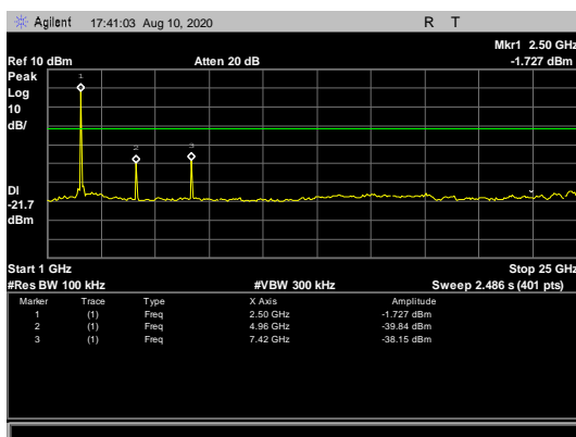
Figure 67: Conducted Spurious Emissions, 2480 MHz - 1-25 GHz
