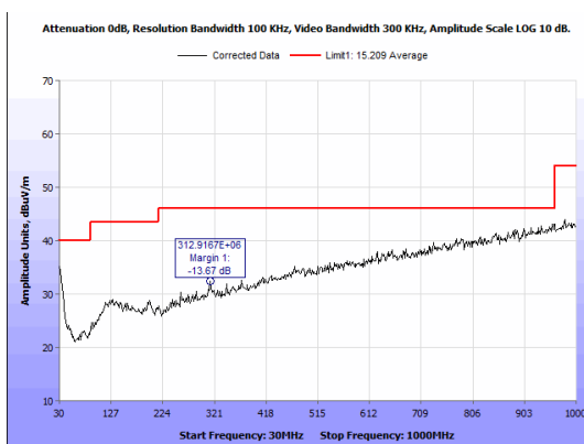
Figure 13: Radiated Emissions, 2402 MHz - 30-1000 MHz - Vertical.
