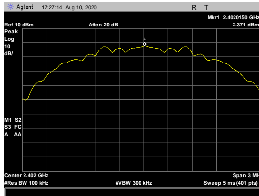
Figure 72: Power Spectral Density, 2402 MHz - (-2.371 dBm)
