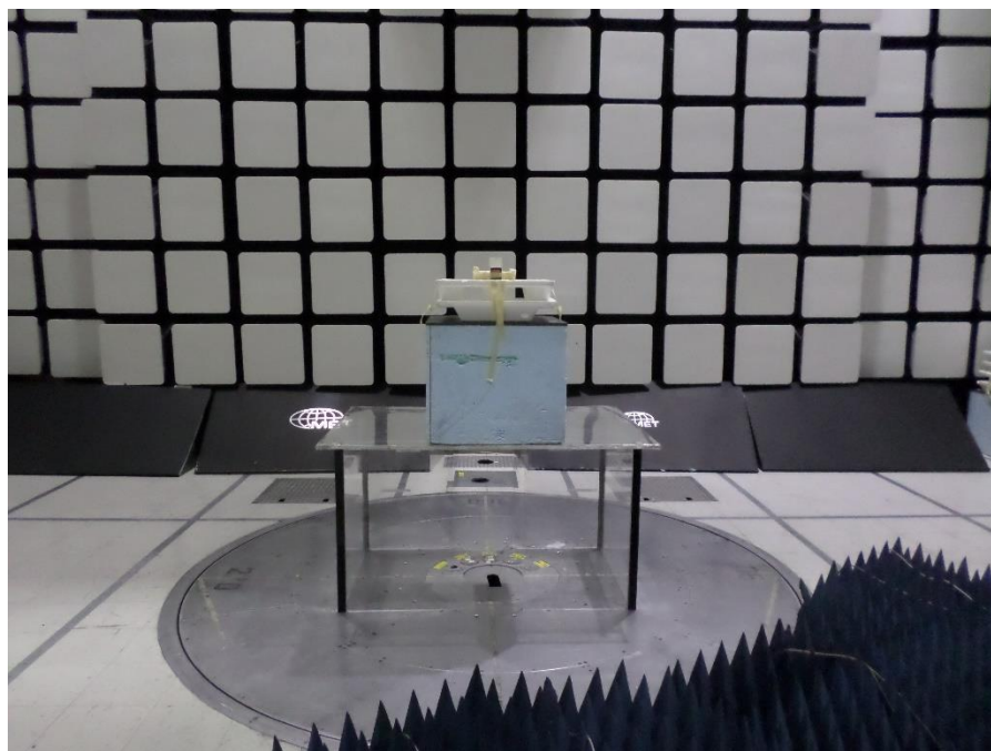
Figure 60: Radiated Emissions, 18-25 GHz - Setup Front View
