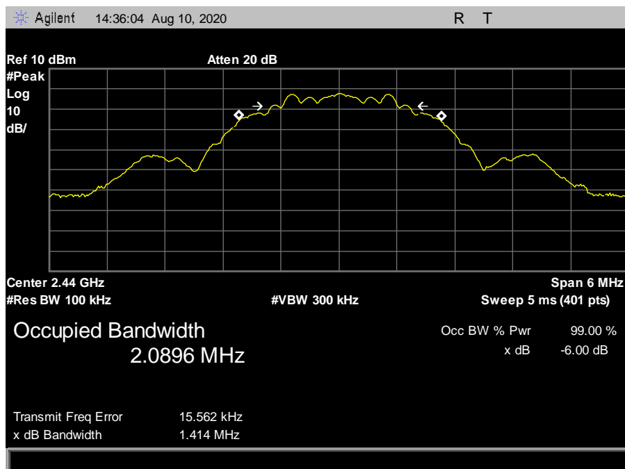
Figure 5: 6 dB Occupied Bandwidth, 2440 MHz - 1.414 MHz
