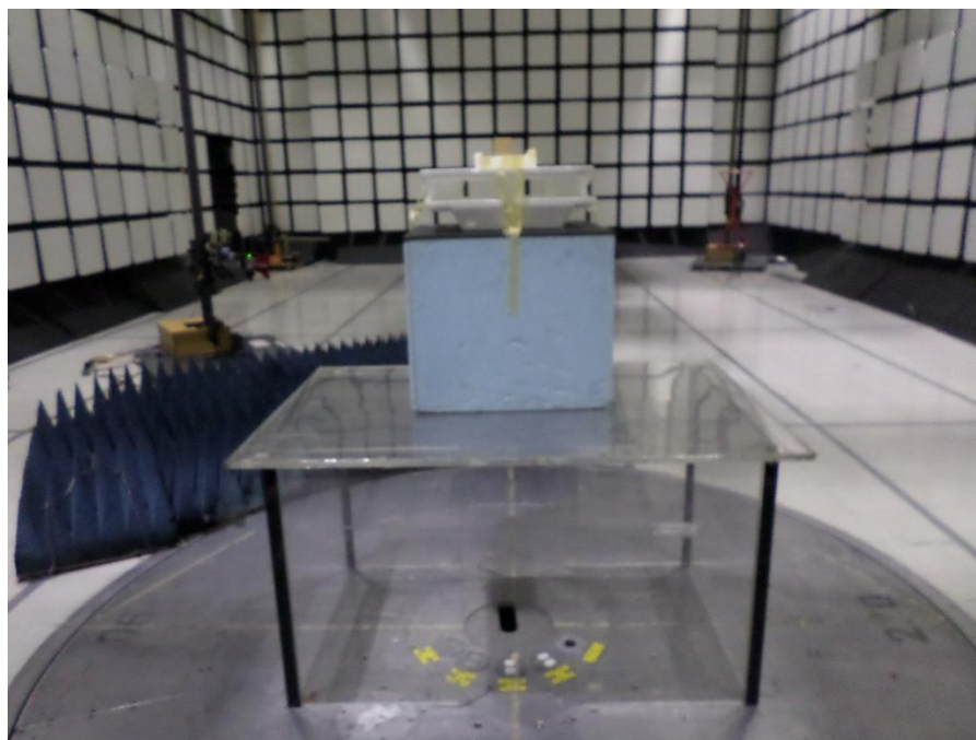
Figure 58: Radiated Emissions, 1-18 GHz - Setup Rear View
