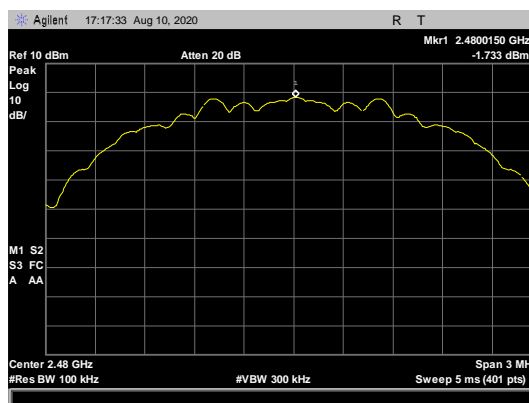
Figure 74: Power Spectral Density, 2480 MHz - (-1.733 dBm)
