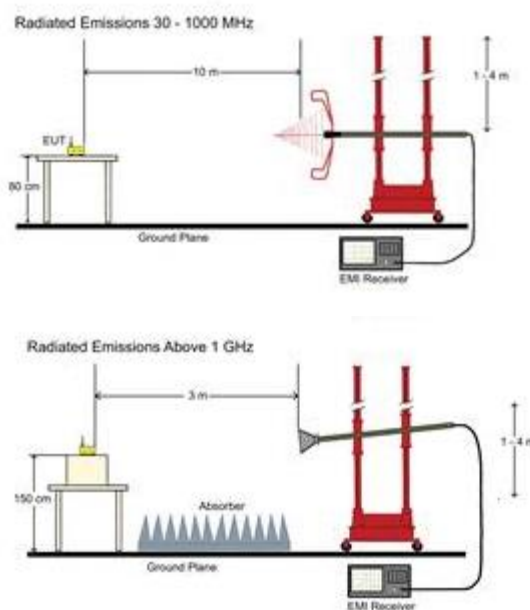
Figure 11: Radiated Emissions Test Setup
