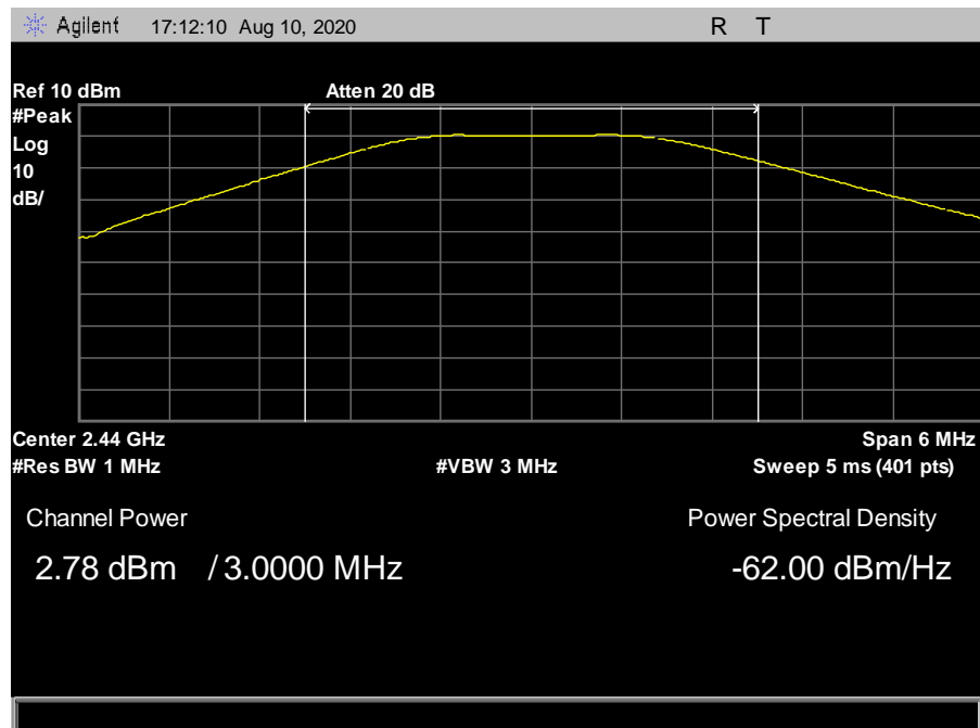
Figure 8: Conducted Output Power, 2440 MHz - (2.78 dBm)
