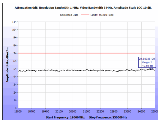
Figure 46: Radiated Emissions, 2480 MHz - 18-25 GHz - Peak - Vertical.
