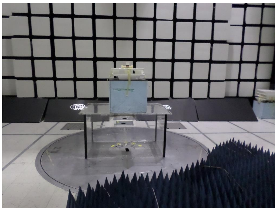
Figure 57: Radiated Emissions, 1-18 GHz - Setup Front View
