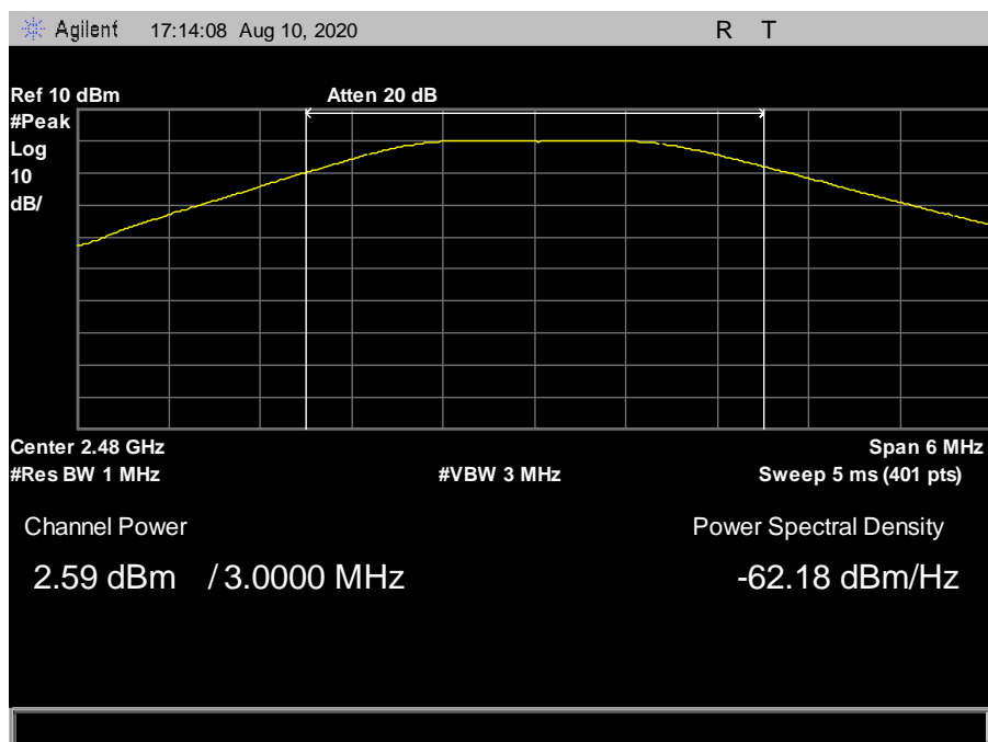
Figure 9: Conducted Output Power, 2480 MHz - (2.59 dBm)
