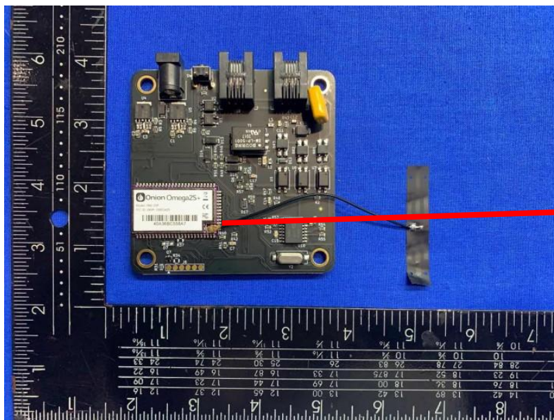
WIFI Antenna
