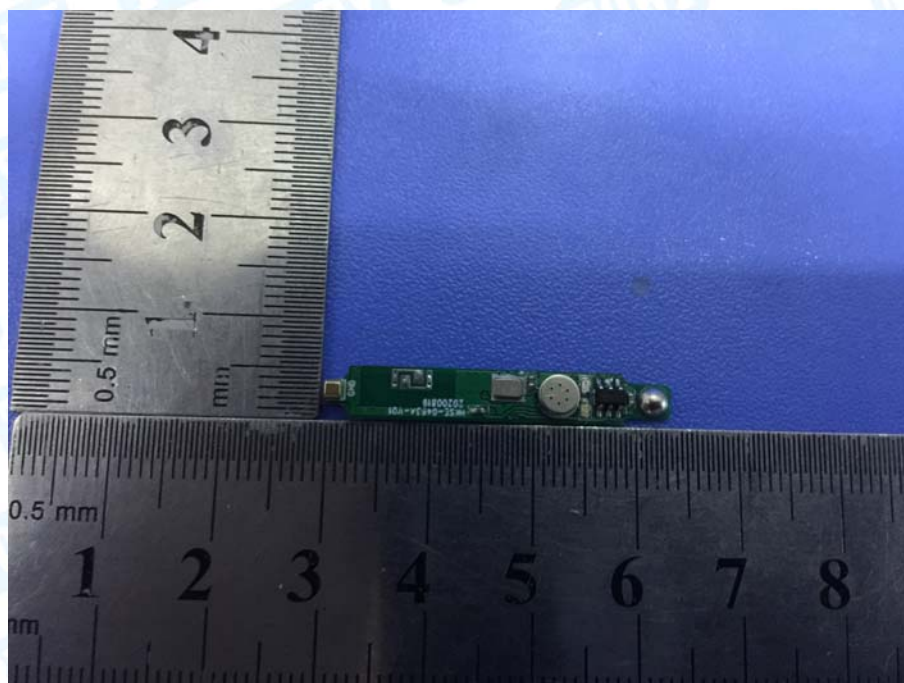
Photo 10 Appearance PCB
