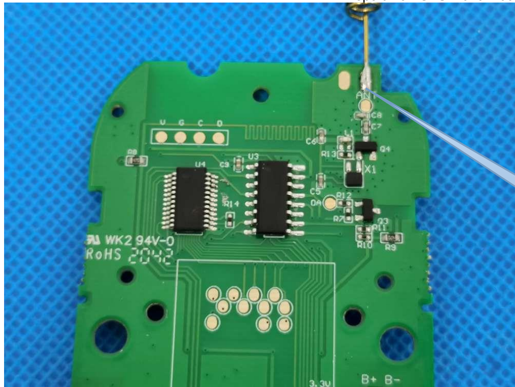
Antenna location
