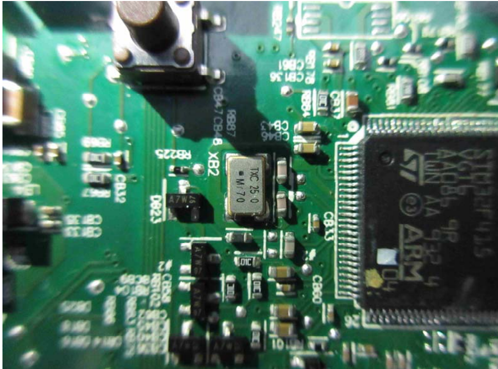
(32) EUT Photo
