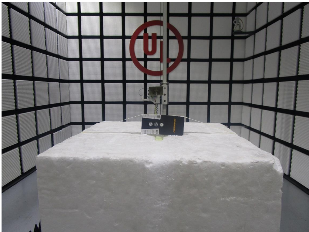
Radiated Disturbance Above 1 GHz (Y axis)
