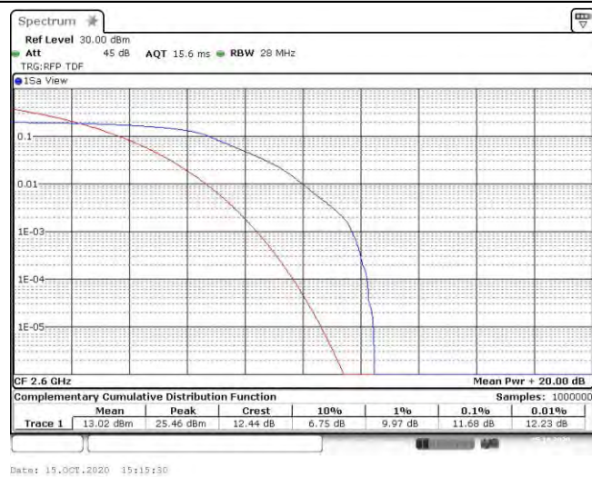
Band41-5MHz-16QAM-41215-25RB#0
