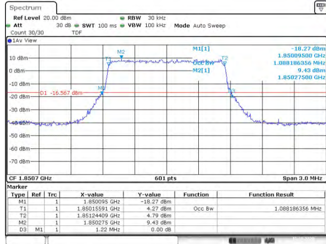
Band25-1.4MHz-QPSK-26047-6RB#0-1.088
