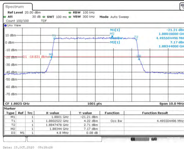
Band25-5MHz-QPSK-26665-25RB#0-4.496
