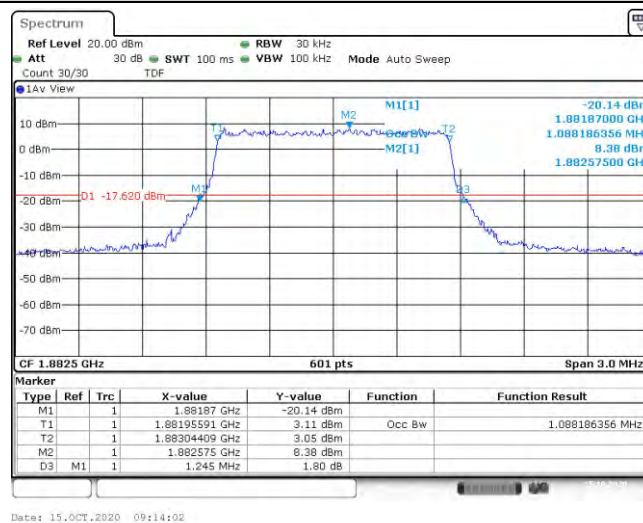
Band25-1.4MHz-16QAM-26683-6RB#0-1.088
