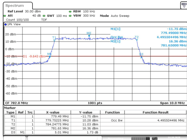
Band13-5MHz-QPSK-23230-25RB#0-4.496
